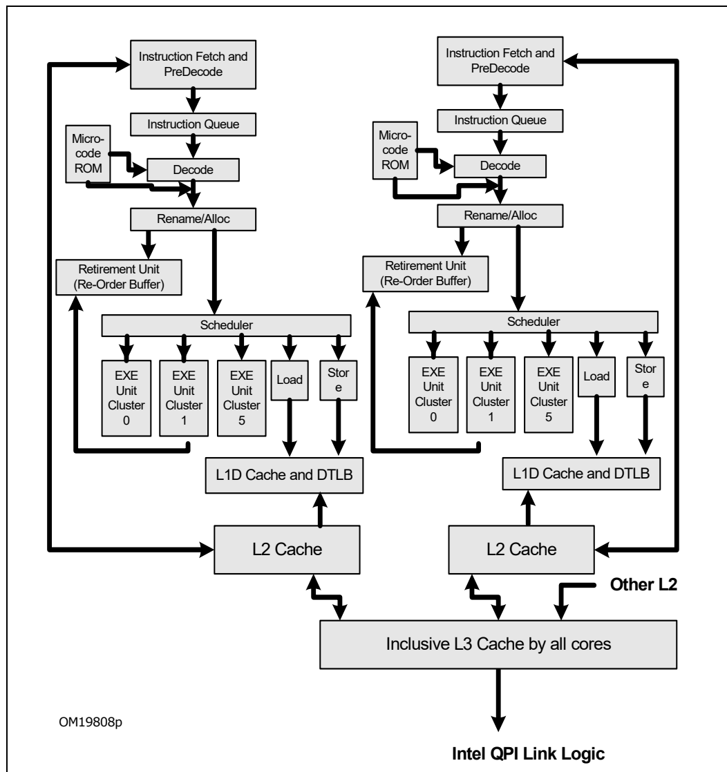
Figure 4-1. Nehalem Microarchitecture Pipeline Functionality
