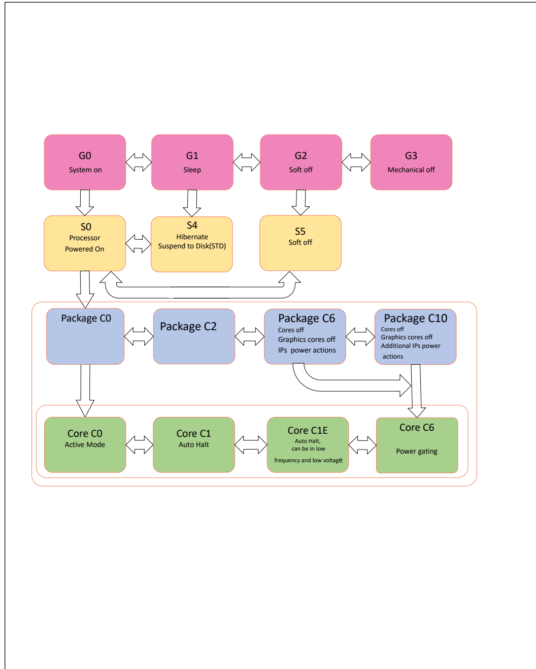
Figure 5. Power State Block Diagram
