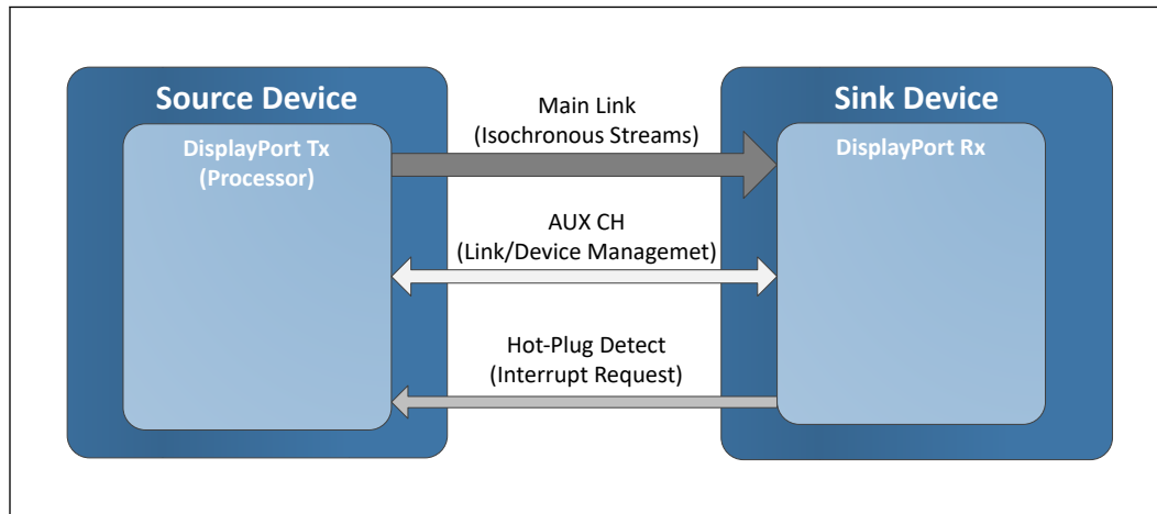
Figure 13. DisplayPort* Overview
