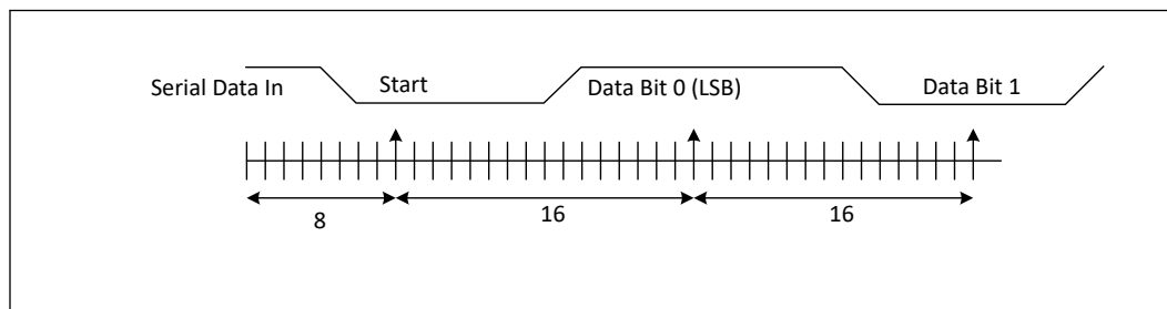
Figure 24. UART Receiver Serial Data Sample Points
