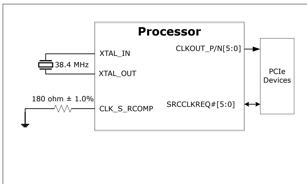
Figure 10. ICC Diagram
