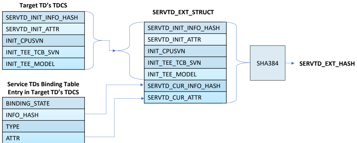
Figure 13.4: SERVTD_EXT_HASH Calculation
