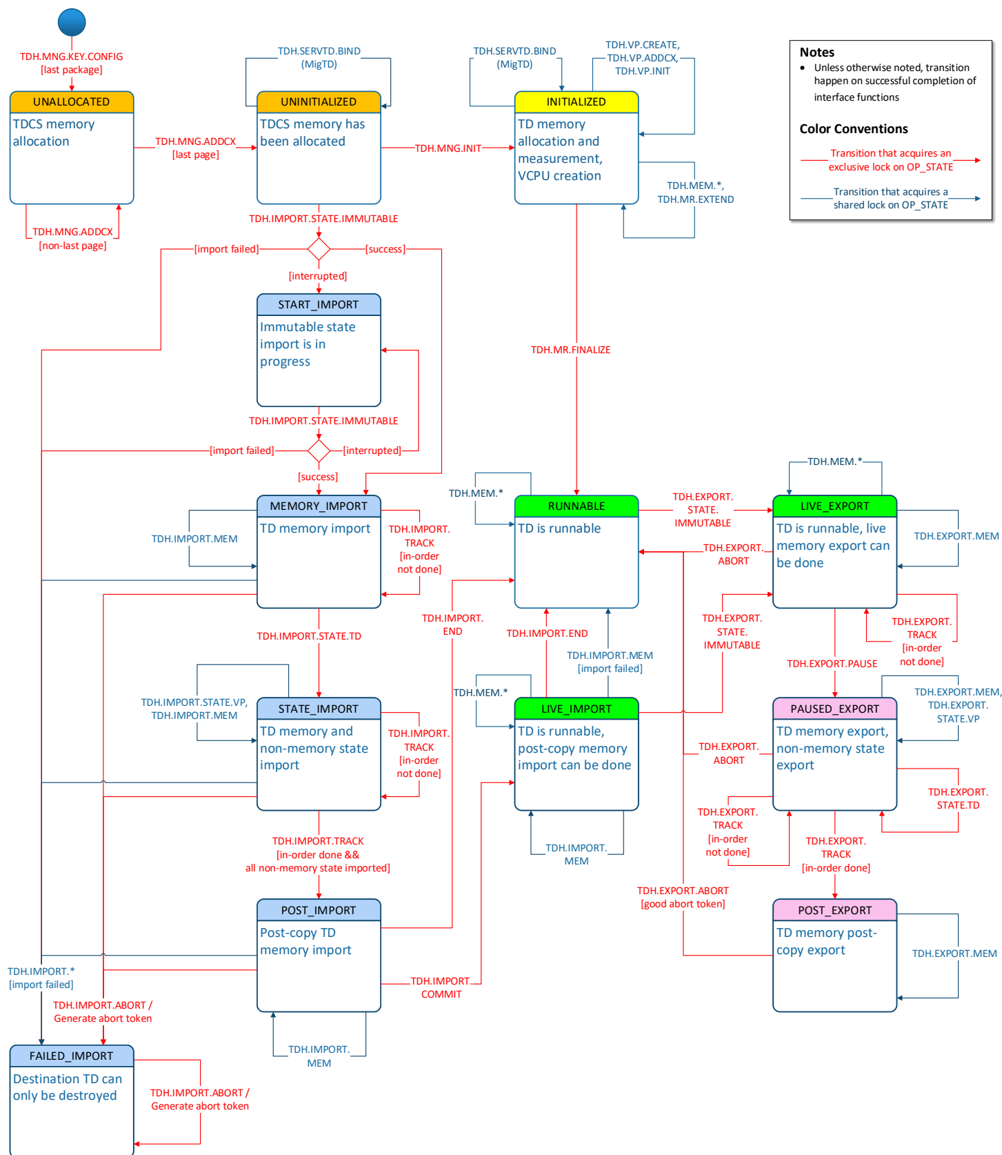
Figure 7.2: TD Operation State Machine (Sub-States of TD_KEYS_CONFIGURED)
