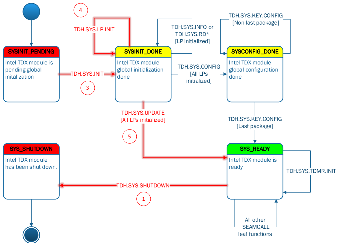
Figure 4.4 the new TDX Module would differ from the old Lifecycle State Machine – TD-Preserving Update
