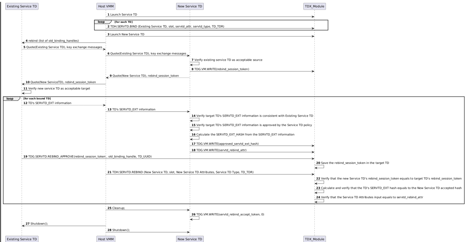
Figure 13.5: Service TD Rebind Flow
