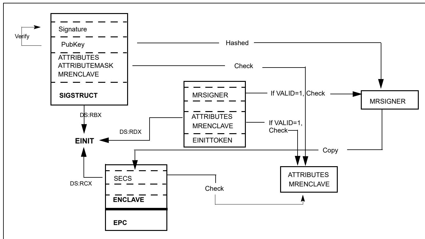
Figure 14-1. Relationships Between SECS, SIGSTRUCT, and EINITTOKEN
