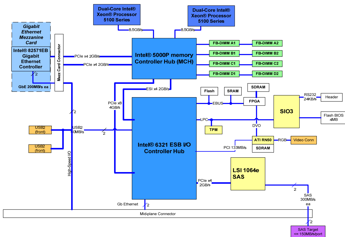
Figure 4. Compute Module Functional Block Diagram
