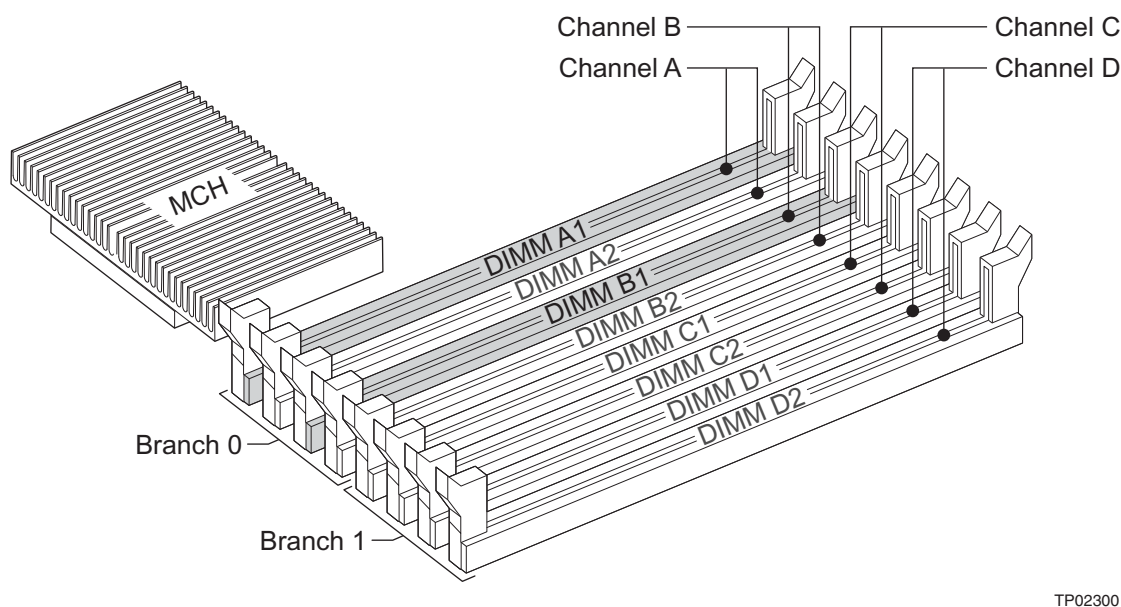
Figure 7. Recommended Minimum Two-DIMM Memory Configuration
