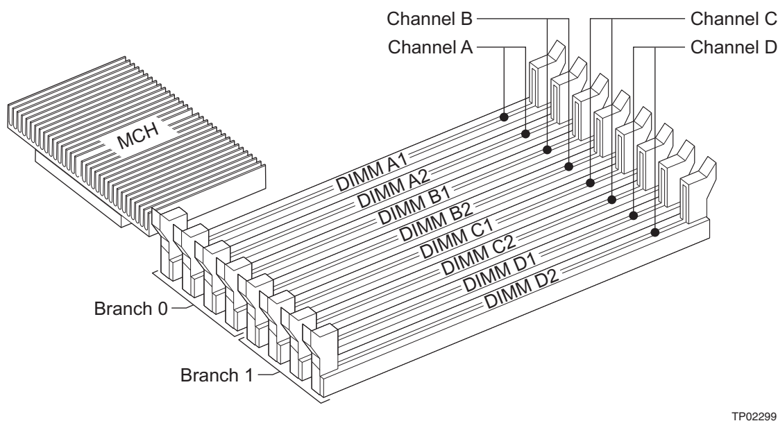
Figure 6. Memory Layout
