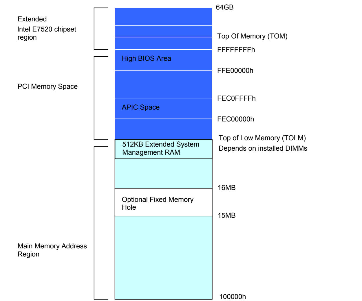
Figure 16. Extended Memory Map
