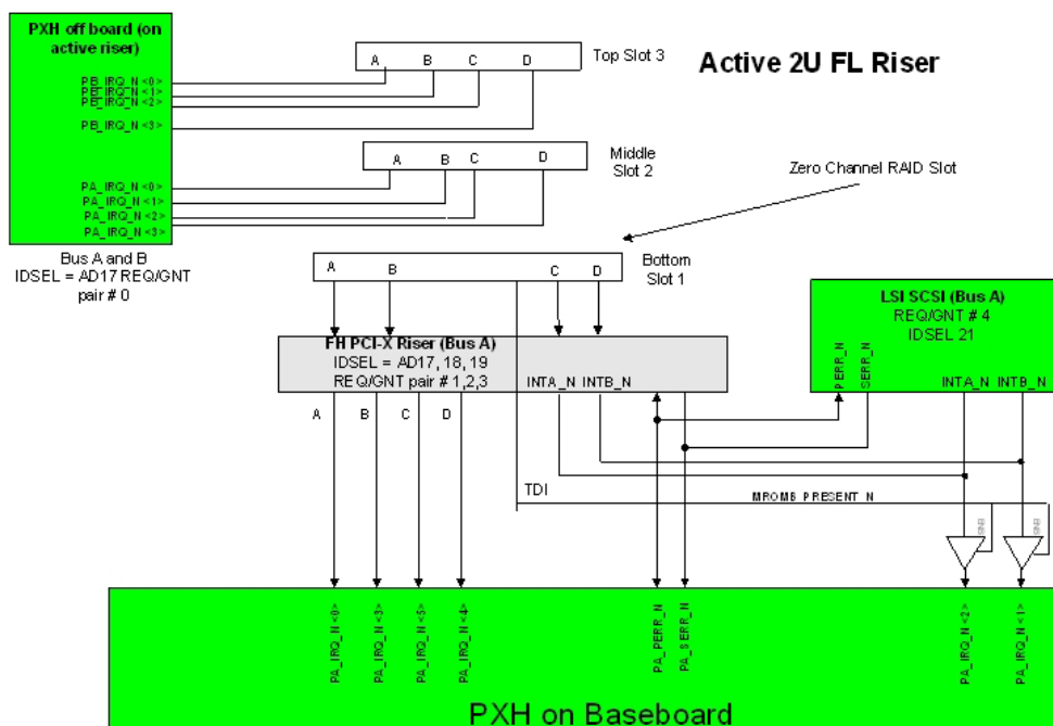
Figure 10. PCI Interrupt Mapping Diagram
