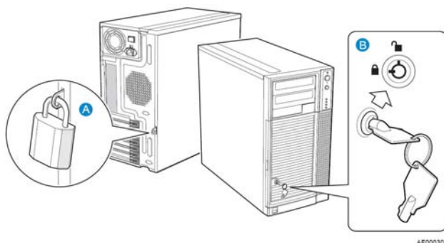
Figure 6. Mechanical Locks
