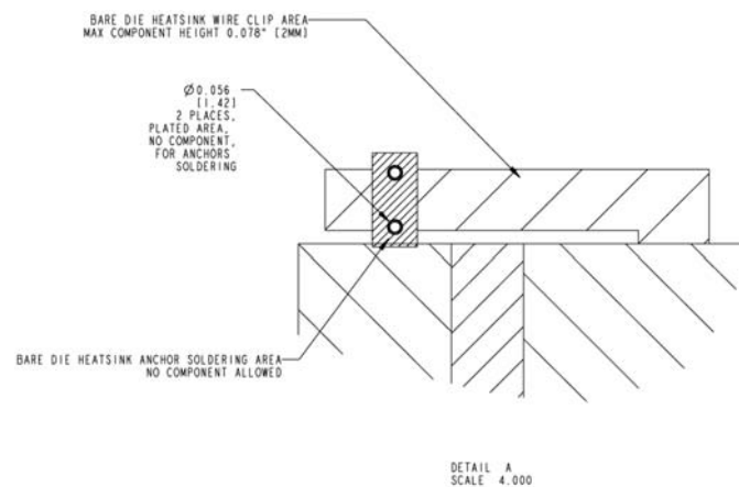
Figure 13. Primary Side Keepout Zone (2 of 2)
