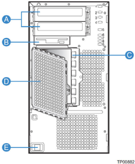
Figure 1. Front View Components (with Front Bezel Assembly)
