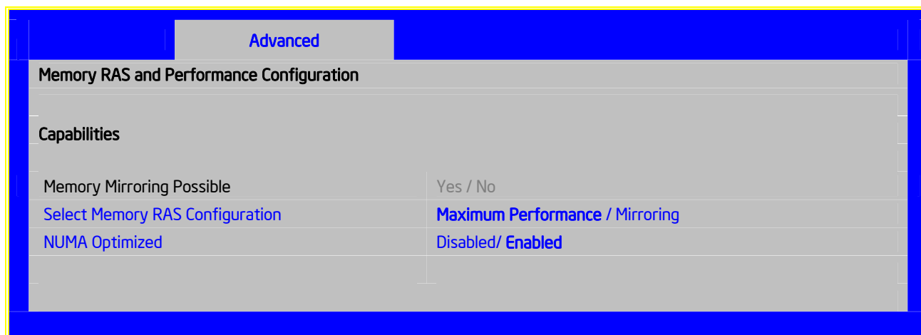
Figure 34. Setup Utility — Configure RAS and Performance Screen Display
