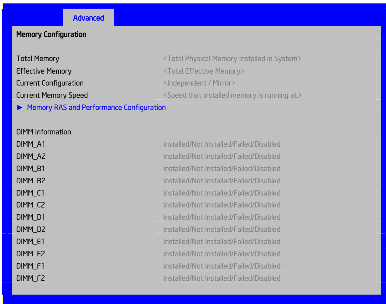
Figure 33. Setup Utility — Memory Configuration Screen Display
