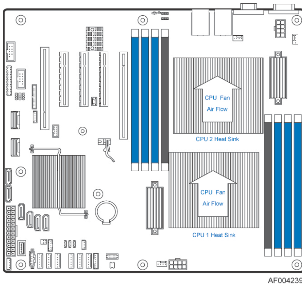
Figure 30. Processor Heatsink Installation
