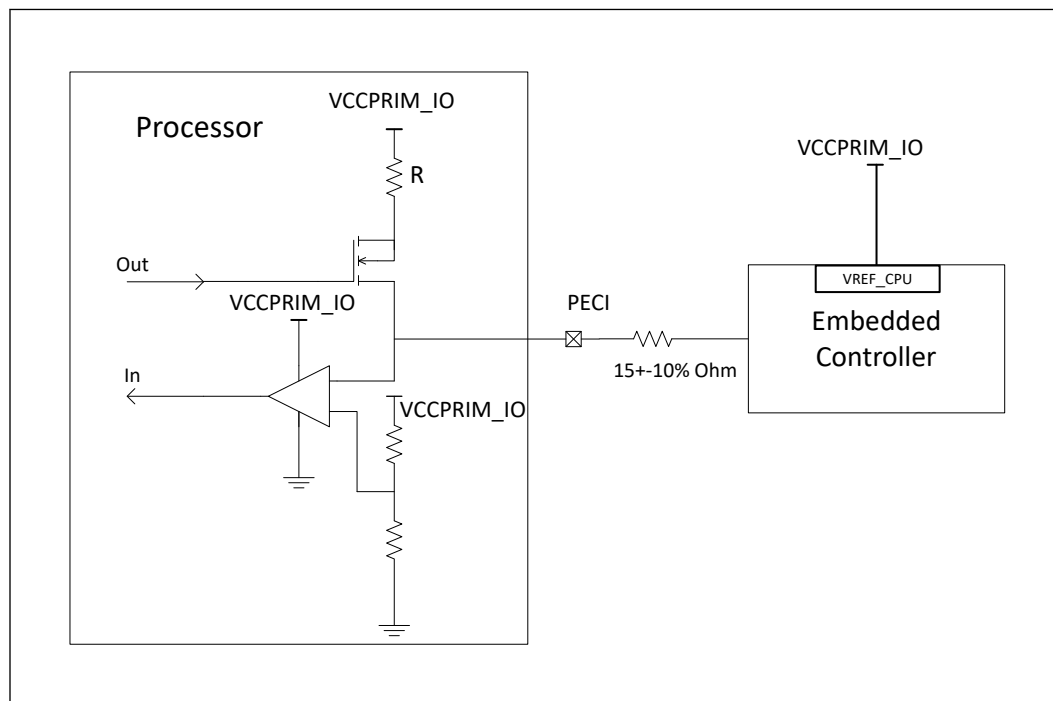
Figure 5. PEFI EC Connection Example
