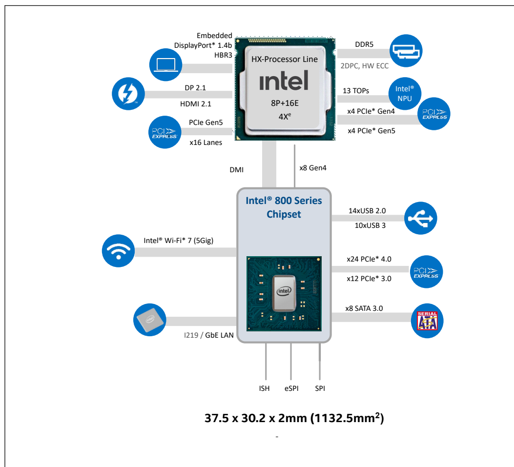
Figure 2. HX Processor Line Platform Diagram
