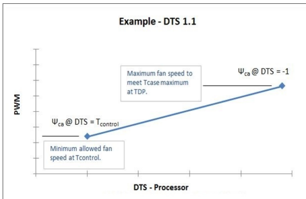
Figure 13. Digital Thermal Sensor (DTS) 1.1 Definition Points
