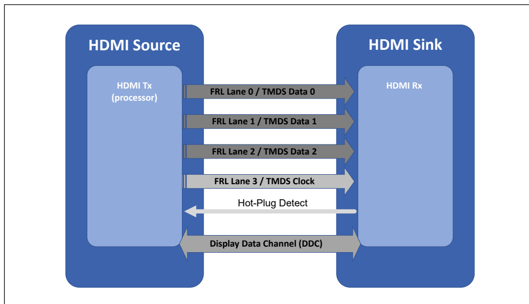
Figure 23. HDMI* Overview
