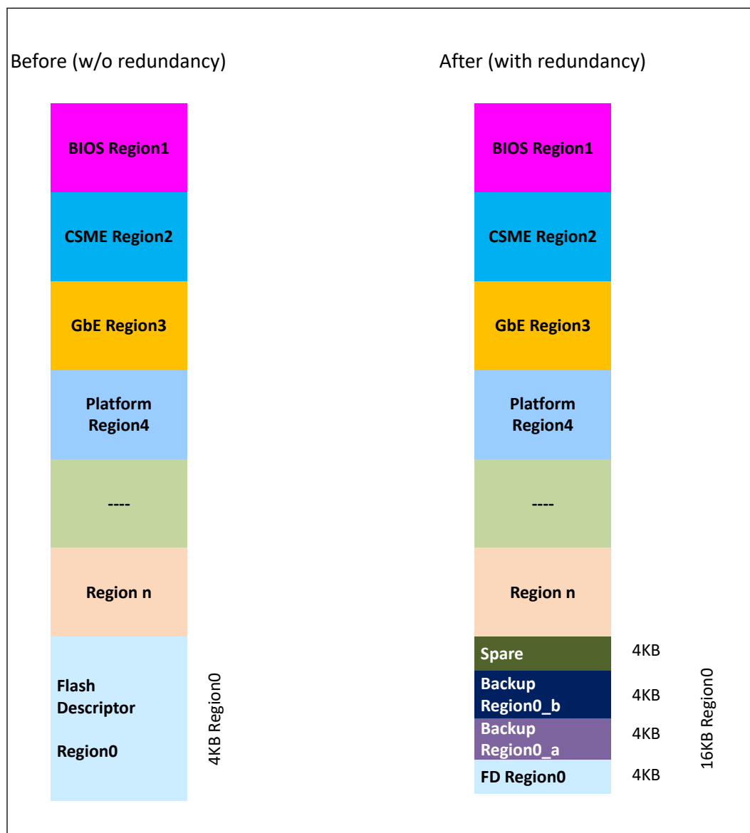
Figure 23. Flash Descriptor Regions
