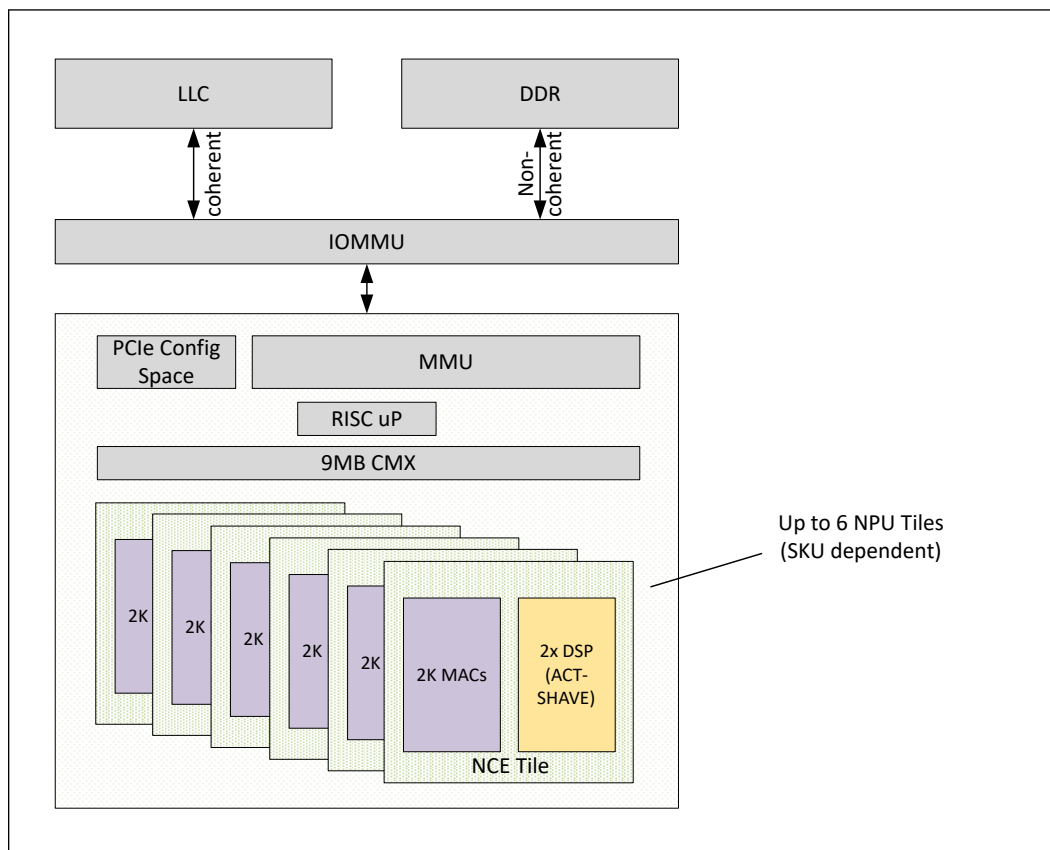
Figure 7. NPU IP Block Diagram
