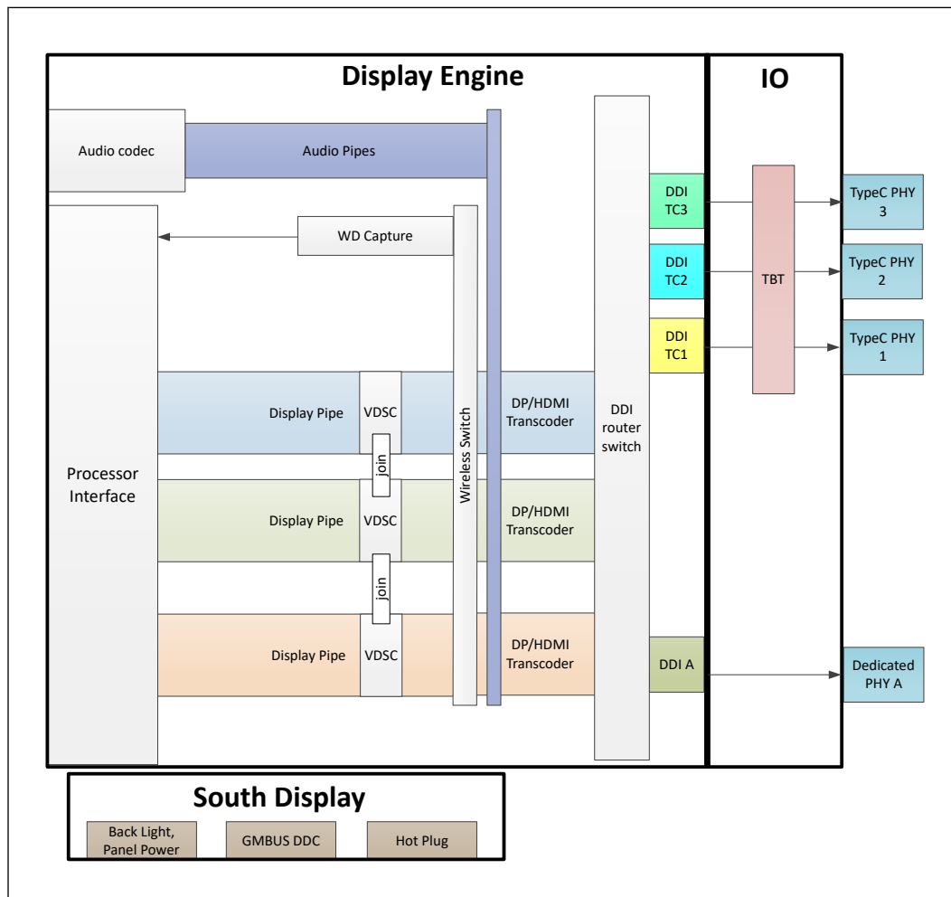
Figure 16. Processor Display Architecture
