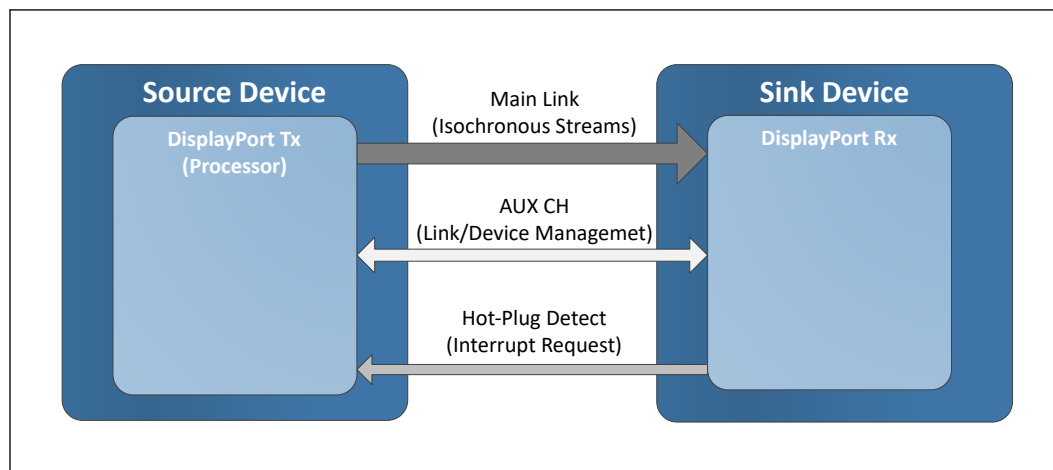
Figure 17. DisplayPort* Overview
