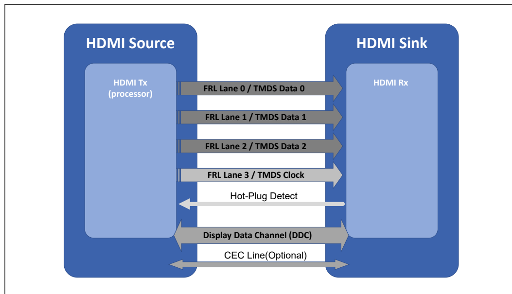
Figure 18. HDMI* Overview
