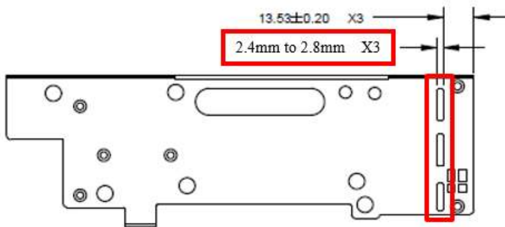
Figure 1. PCIe* Riser Bracket
