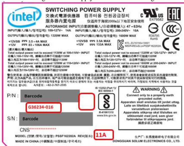
Image 1. Power supply label before the change
