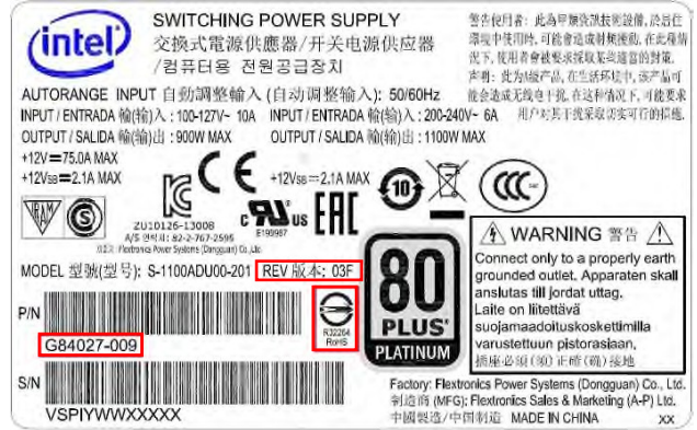
Image 2. Power supply label after change
