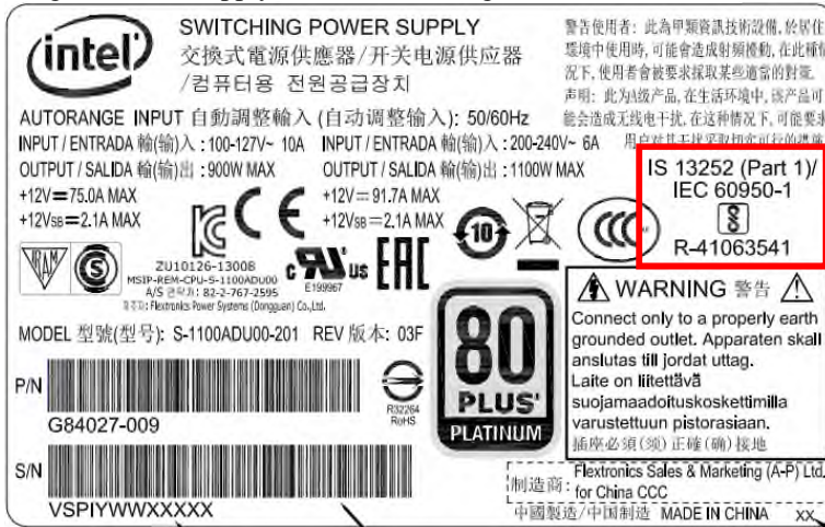
Image 1. Power supply label before change
