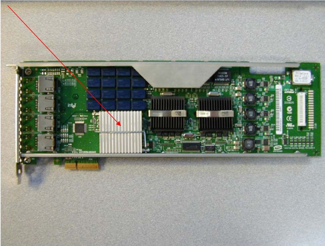
Before picture with Heat Sink and Clip
