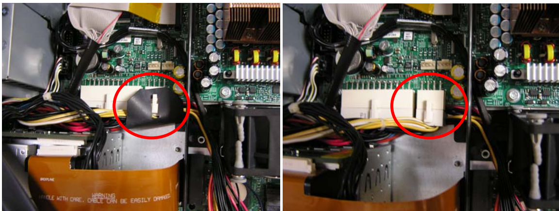
Old design with shield to protect the baseboard power cables.
