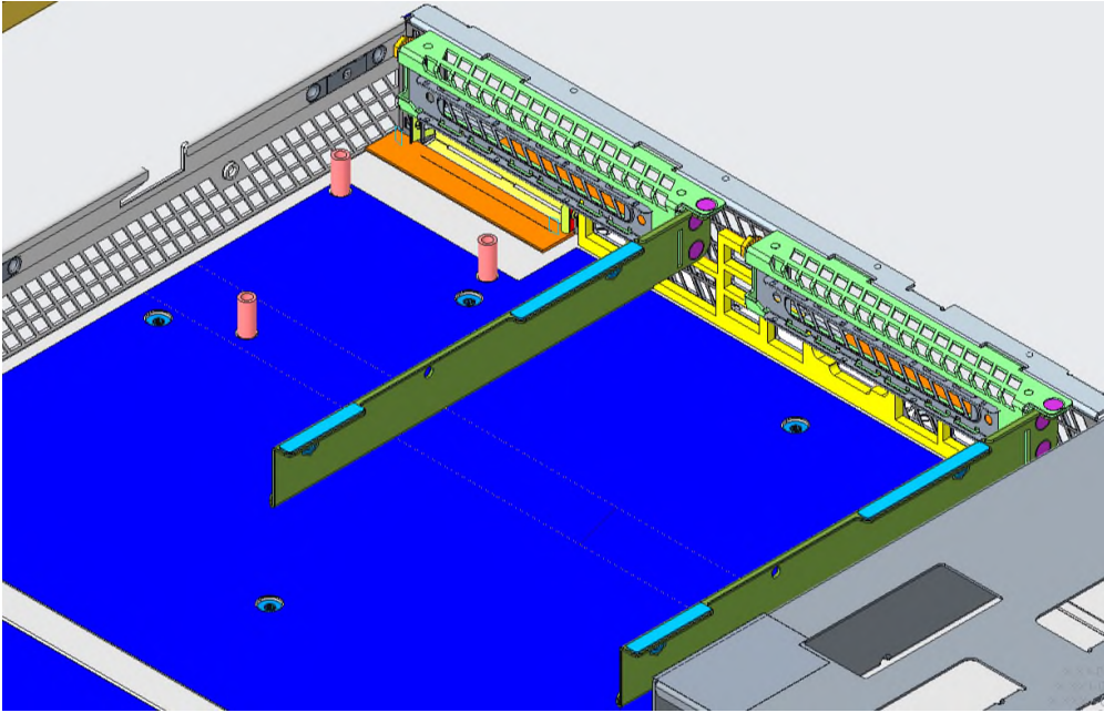
Image 1. Riser bracket before ESD gasket added
