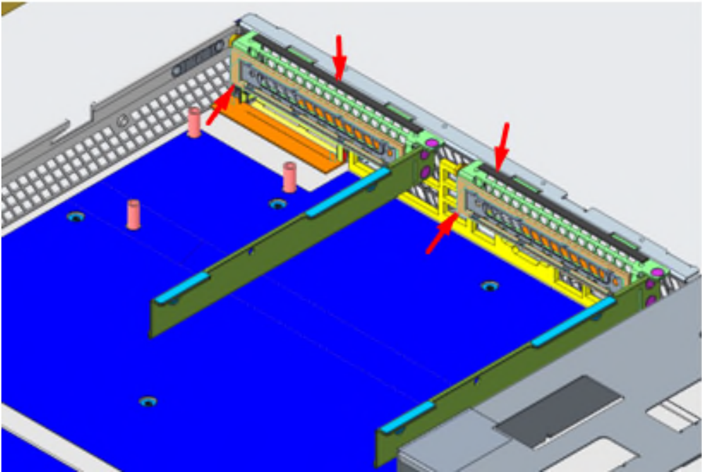
Image 2. Riser bracket after ESD gasket added
