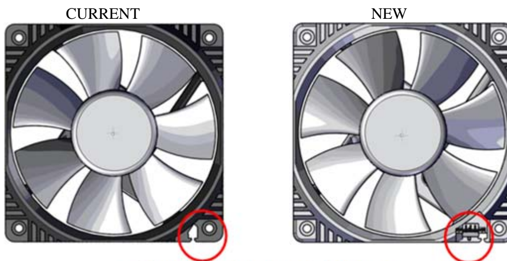
Addition of a switch to turn off the fan LEDs
