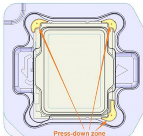
New Clamshell Design
