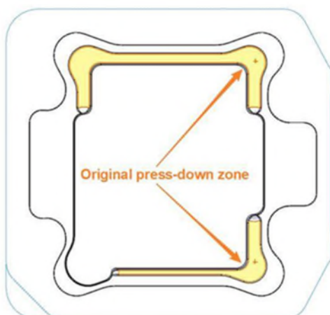
Current Clamshell Design
