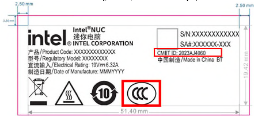
CN L10 Rating Label (first version sample)
