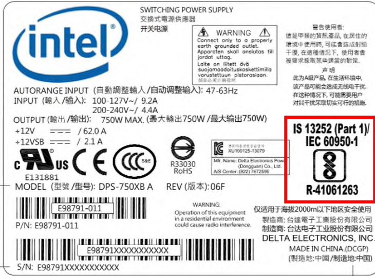
Image 3. Power supply label before change
