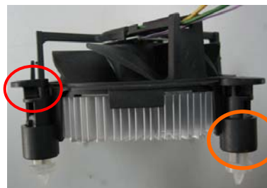
Modified clip-less heatsink for illustration purposes only
