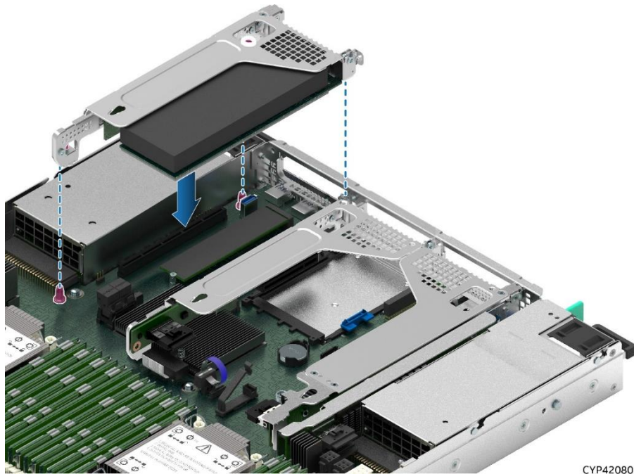
Figure 44. Add-in Card Placement into Server System Chassis
