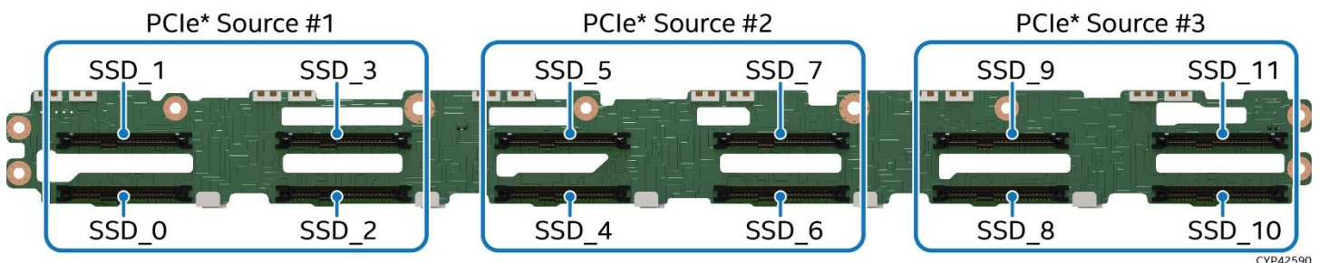
Figure 83. 12 x 2.5" SAS/SATA/NVMe* Hot Swap Backplane – Front Side
