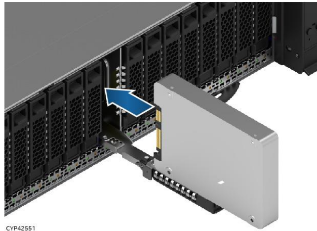
Figure 65. 15 mm Drive Insertion into 2.5" Drive Bay, Ready to Install
