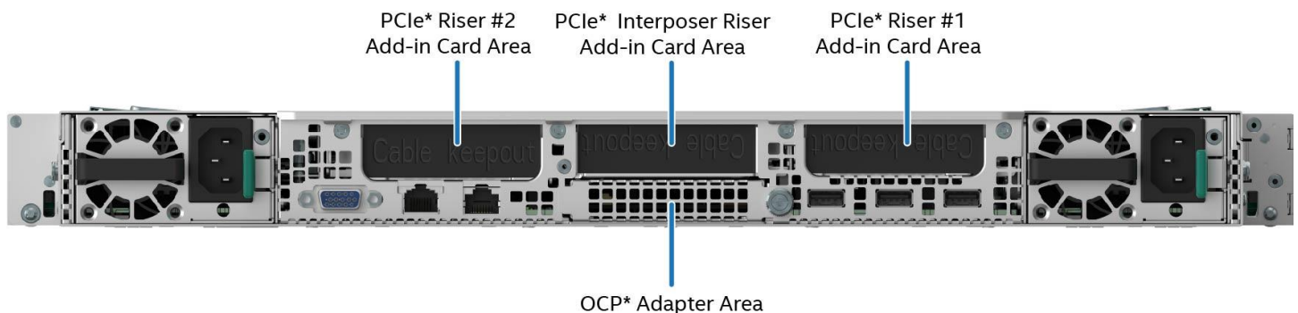
Figure 41. Server System Back Bay Add-in Card Areas
