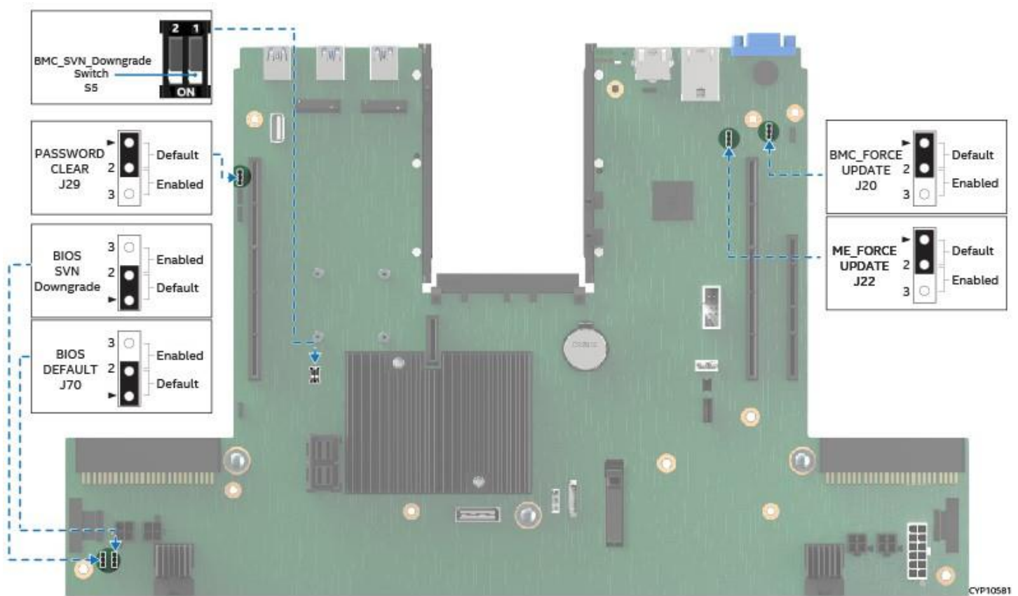
Figure 11. System Configuration and Recovery Jumpers
