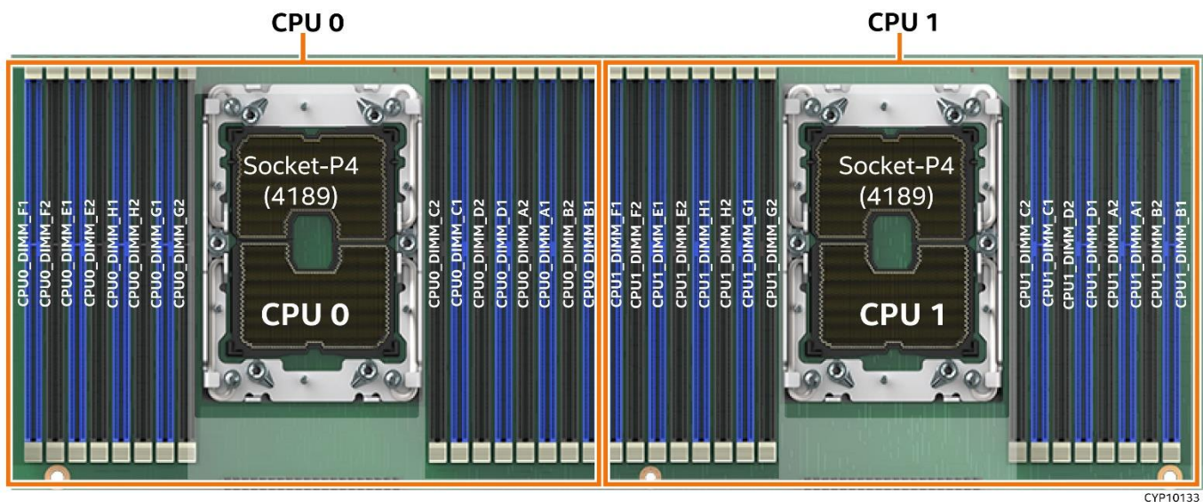
Figure 29. Memory Slot Layout
