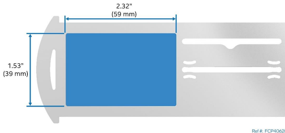
Figure 15. Pull-out Tab Label Emboss Dimensions
