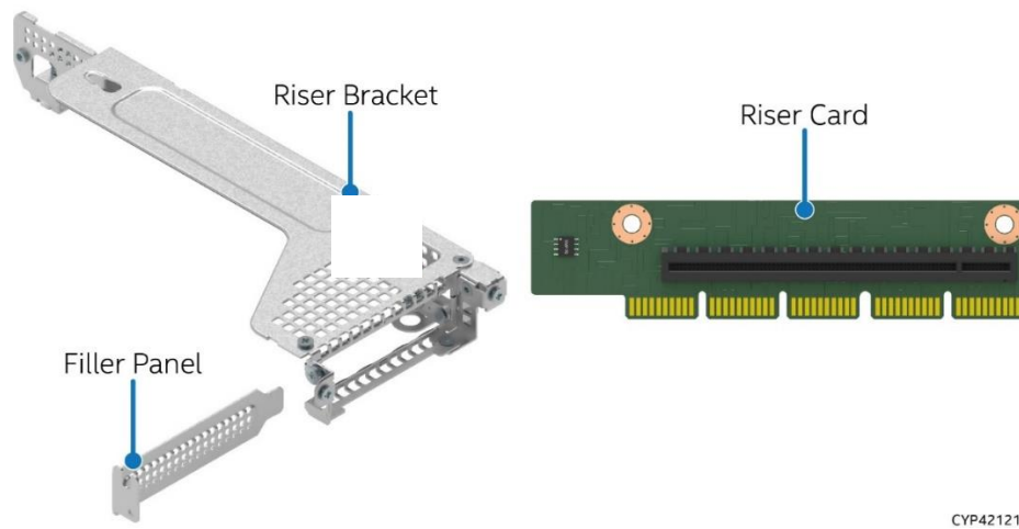
Figure 43. Riser Bracket Components
