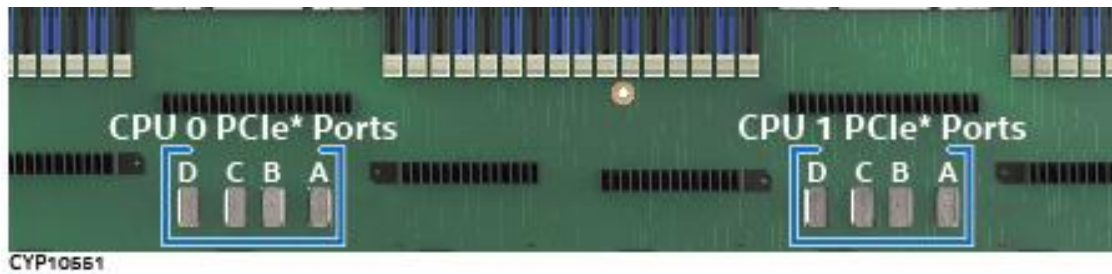
Figure 76. PCIe SlimSAS Connectors
