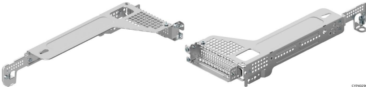
Figure 48. Bracket for PCIe* Interposer Riser Card – Two Views
