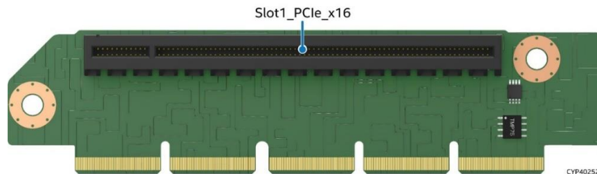
Figure 50. PCIe* Riser Card for Riser Slot #2
