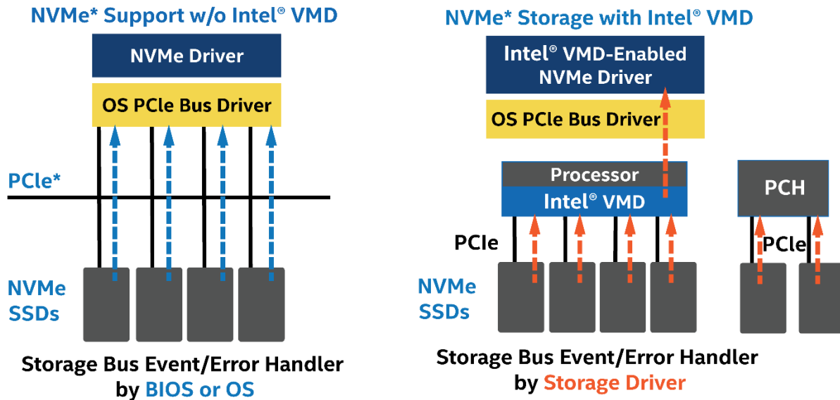
Figure 79. NVMe* Storage Bus Event / Error Handling
