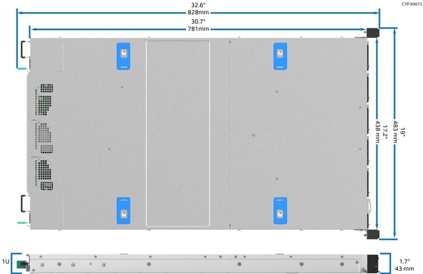
Figure 12. Chassis Dimensions
