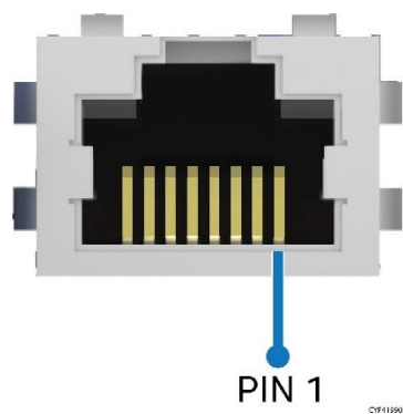
Figure 96. RJ45 Serial Port A Pin Orientation
