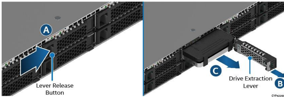
Figure 64. 7 mm Drive Removal from 2.5" Drive Bay
