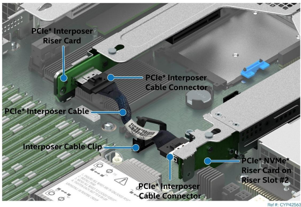
Figure 53. PCIe* Interposer Riser Card to PCIe* NVMe* Riser Card Connectivity
