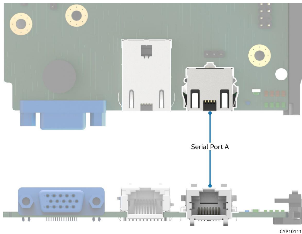
Figure 95. Serial Port A
