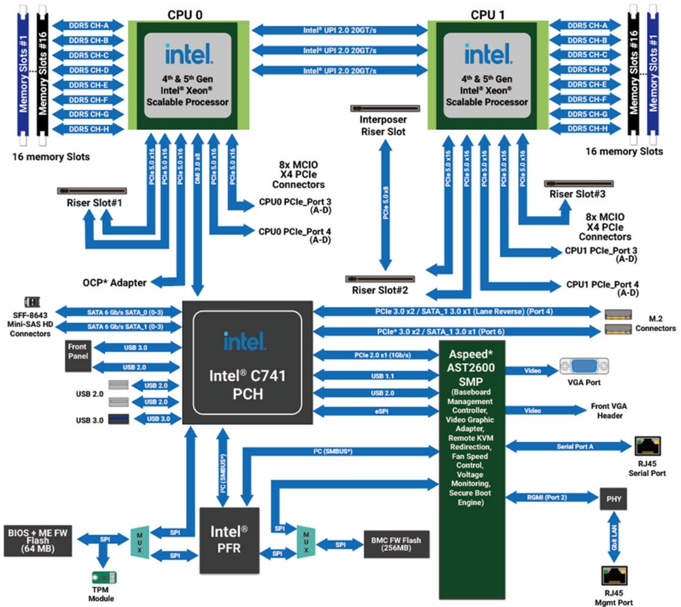
Figure 13. Intel® Server Board M50FCP2SBSTD Architectural Block Diagram
