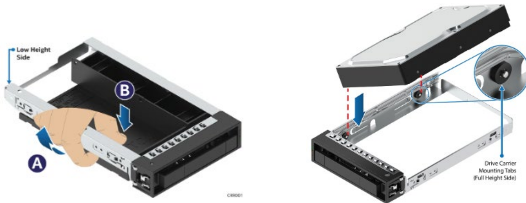
Figure 65. 3.5" Drive Assembly
