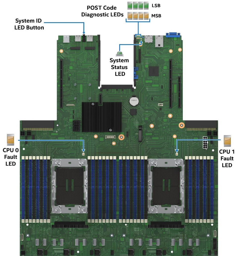
Figure 15. Intel® Light-Guided Diagnostics – LED Identification
