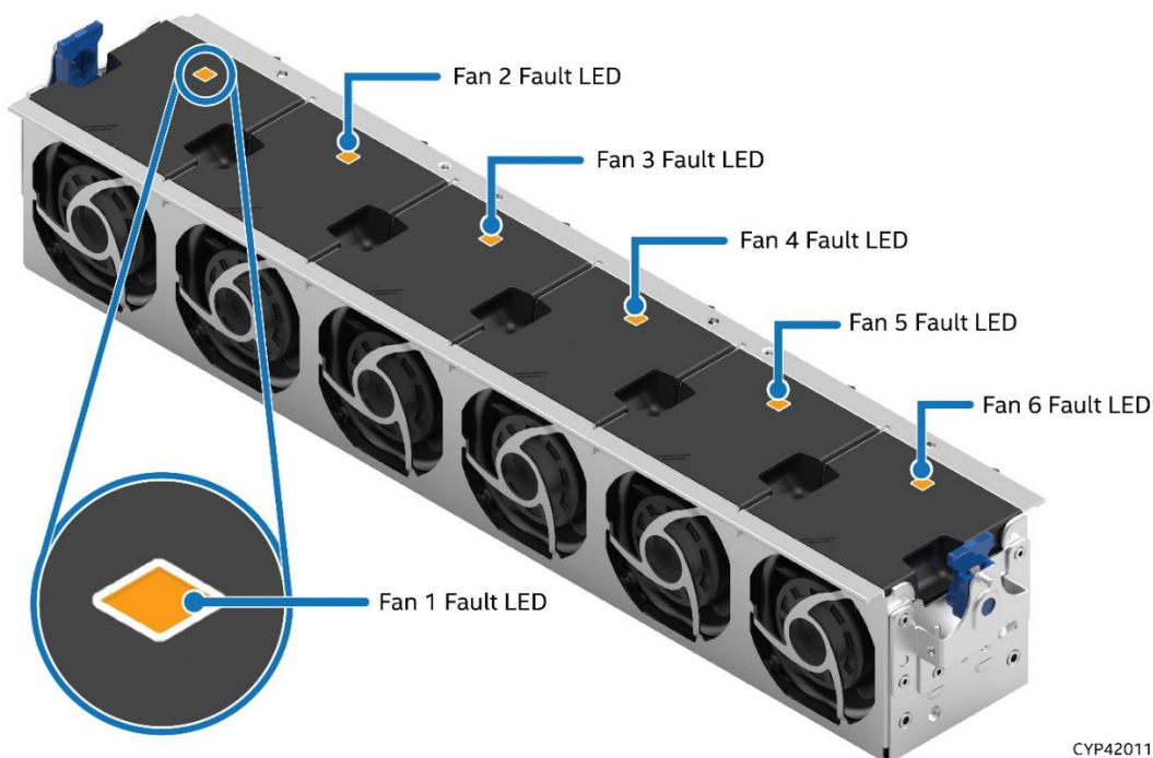
Figure 104. Fan Fault LED Location
