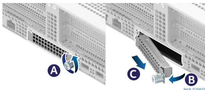
Figure 57. OCP* Adapter Bay Filler Removal
