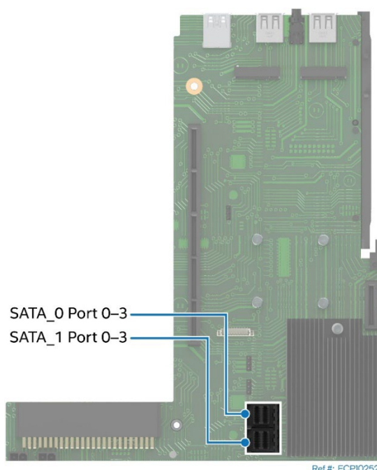
Figure 92. Onboard SATA Port Connectors
