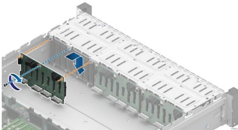
Figure 69. 2.5" Backplane Placement
