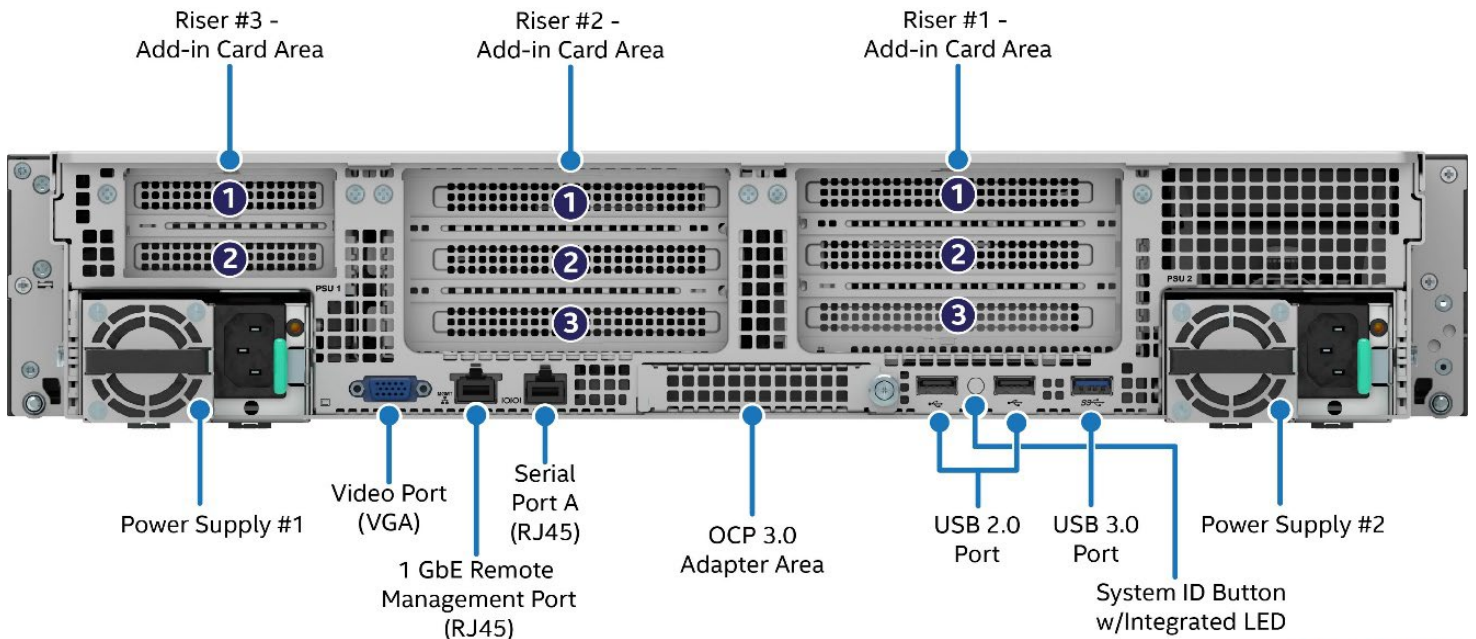
Figure 5. Back Panel Feature Identification
