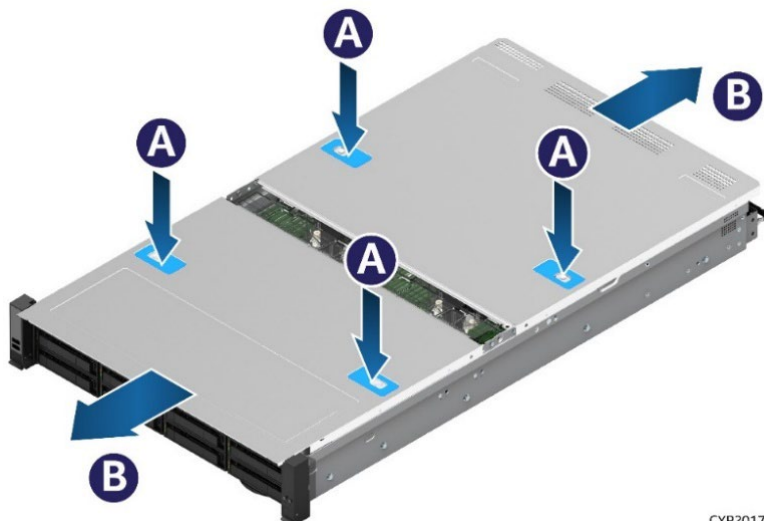
Figure 24. System Top Cover Removal
