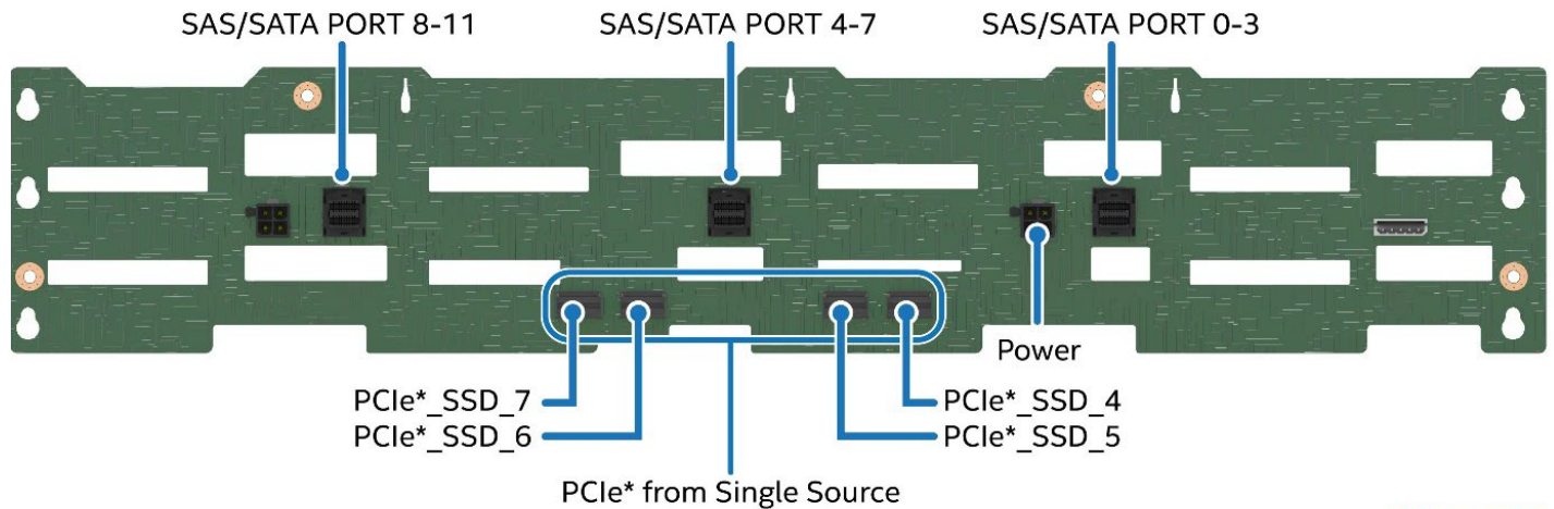
Figure 88. 12 x 3.5" HSBP Connector Identification – Back Side
