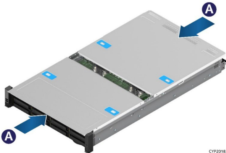
Figure 25. System Top Cover Installation
