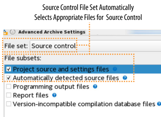
Figure 33. Advanced Archive Settings Dialog Box
