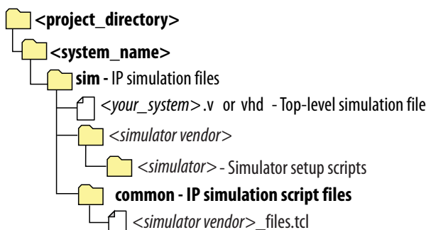
Figure 58. Generated Simulation Files Location
