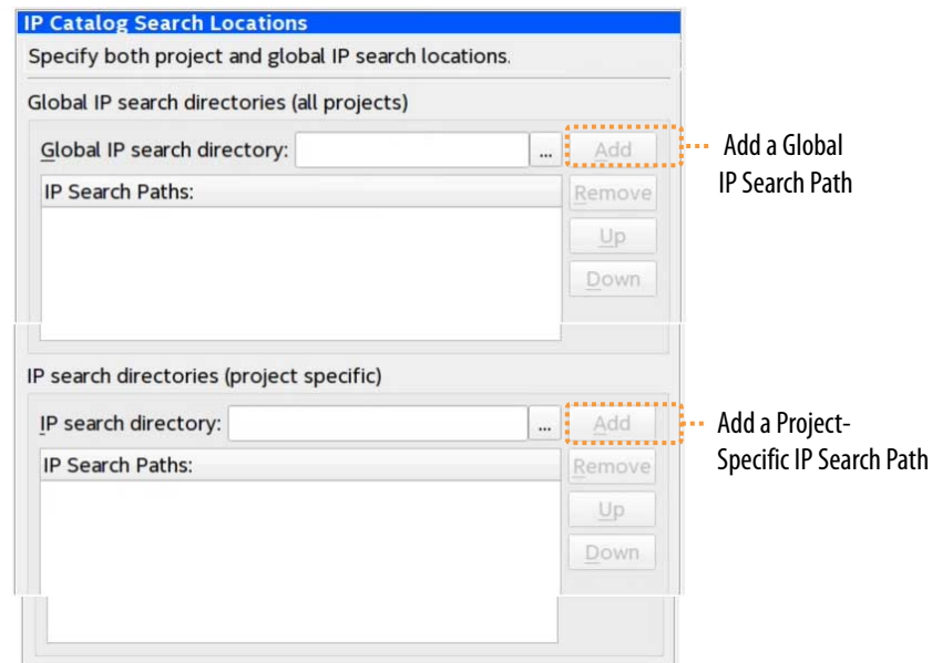
Figure 46. Specifying IP Search Locations
