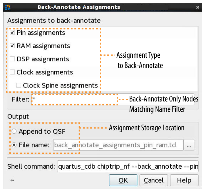
Figure 17. Back-Annotate Assignments Dialog Box
