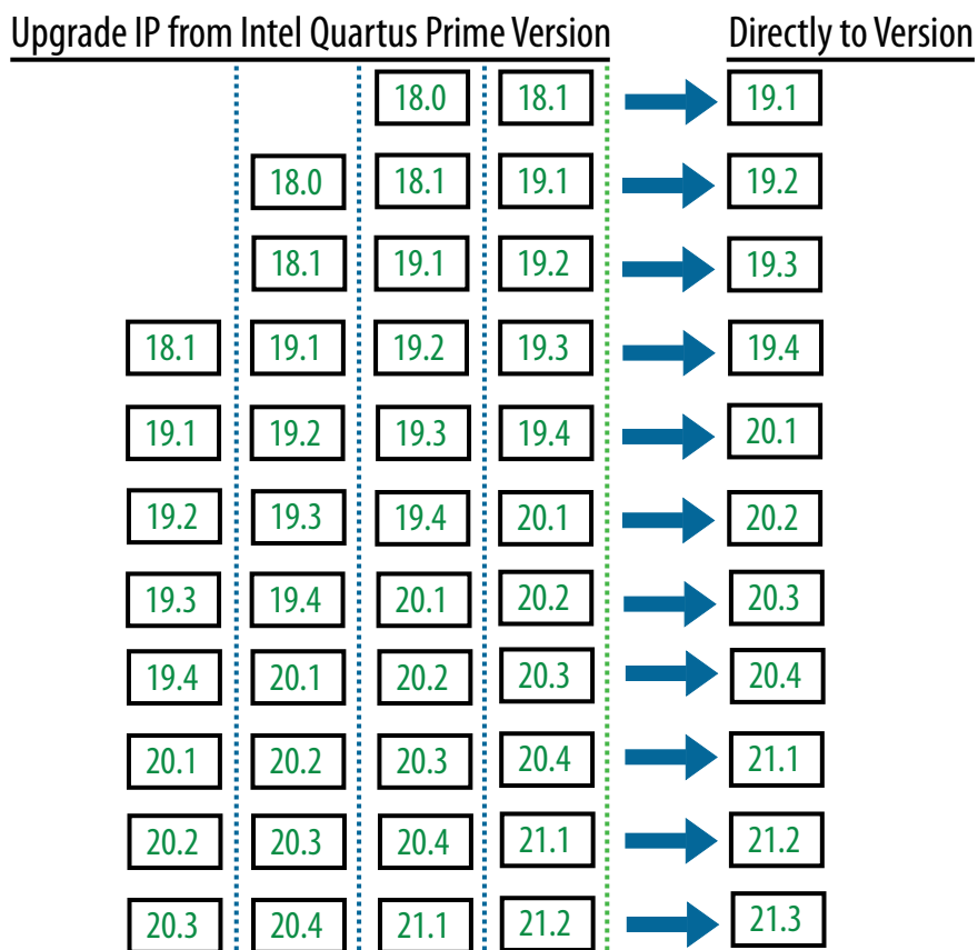
Figure 51. Intel Quartus Prime Pro Edition IP Version Upgrade Paths
