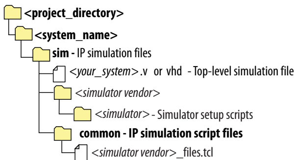
Figure 55. Generated Simulation Files Location
