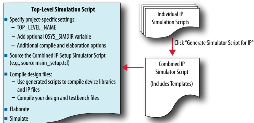
Figure 56. Incorporating Generated Simulator Setup Scripts into a Top-Level Simulation Script
