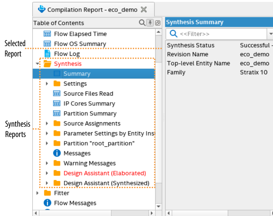
Figure 7. Compilation Report
