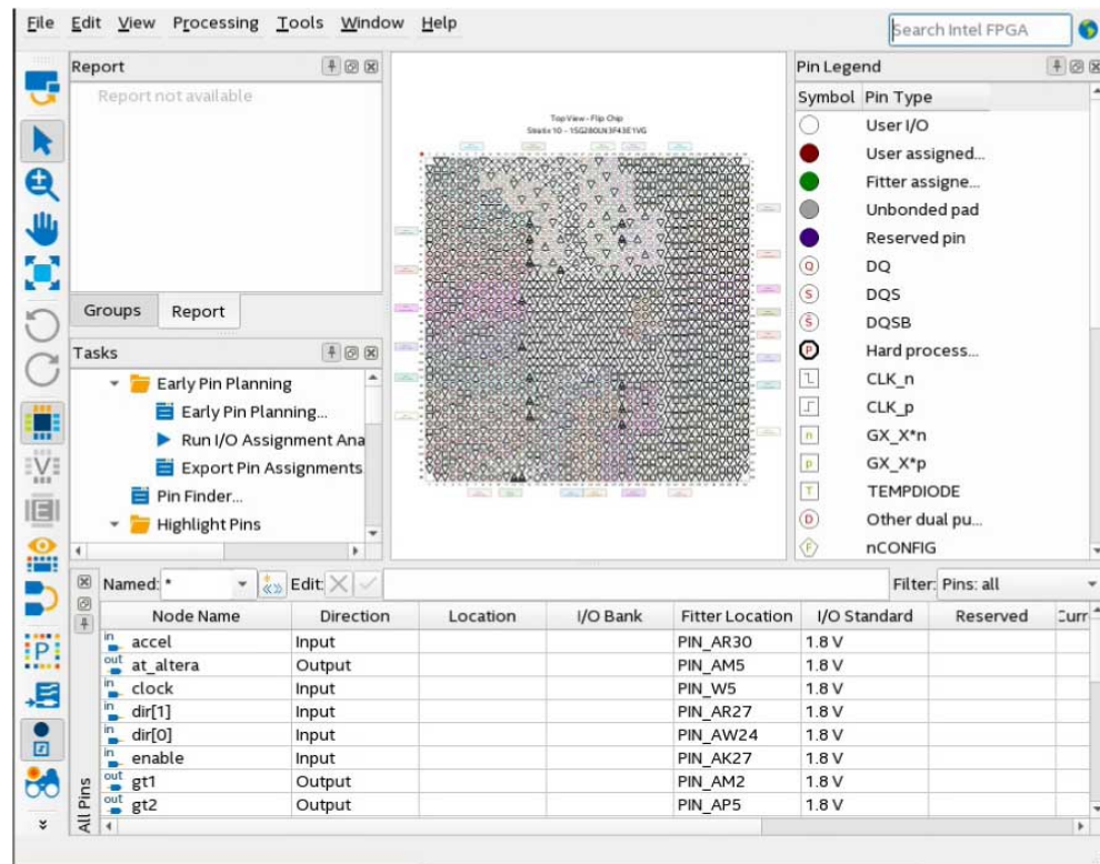
Figure 39. Pin Planner
