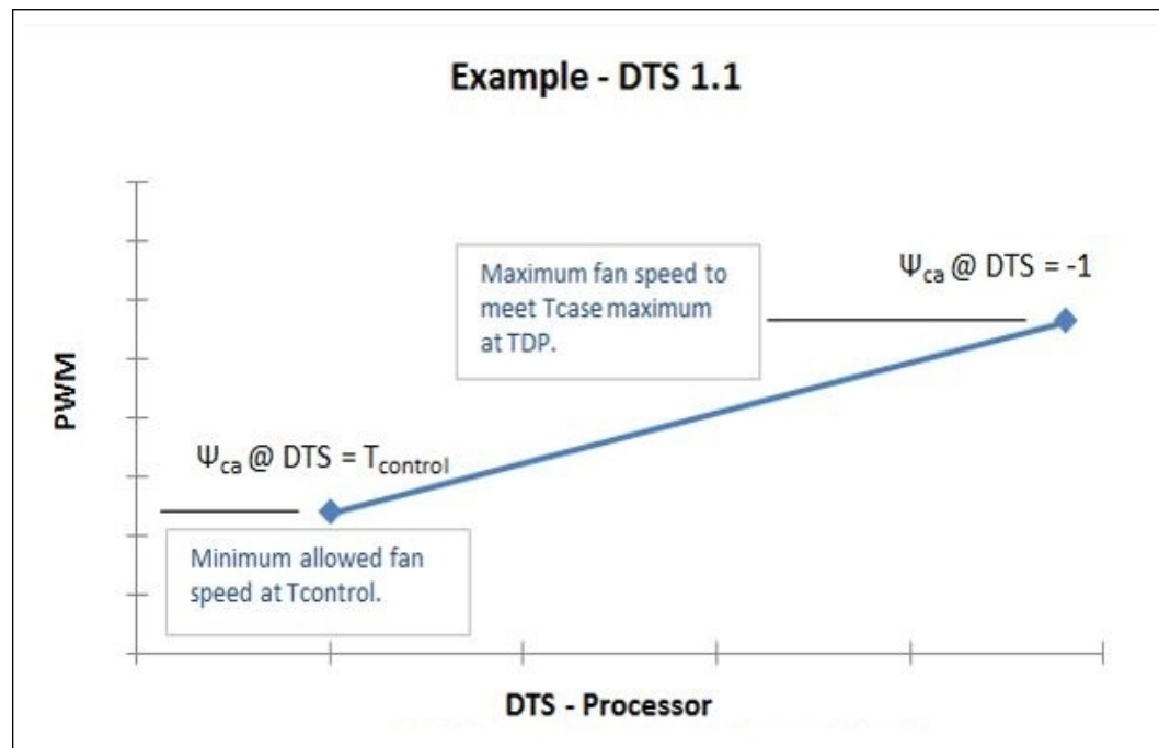
Figure 23. Digital Thermal Sensor (DTS) 1.1 Definition Points
