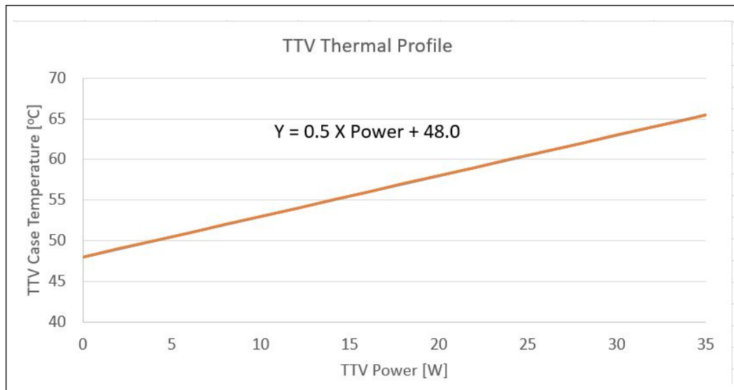
Figure 21. Thermal Test Vehicle Thermal Profile for PCG 2020D Processor
