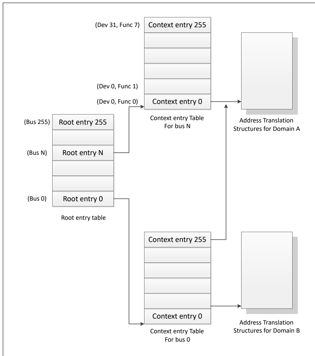
Figure 8. Device to Domain Mapping Structures
