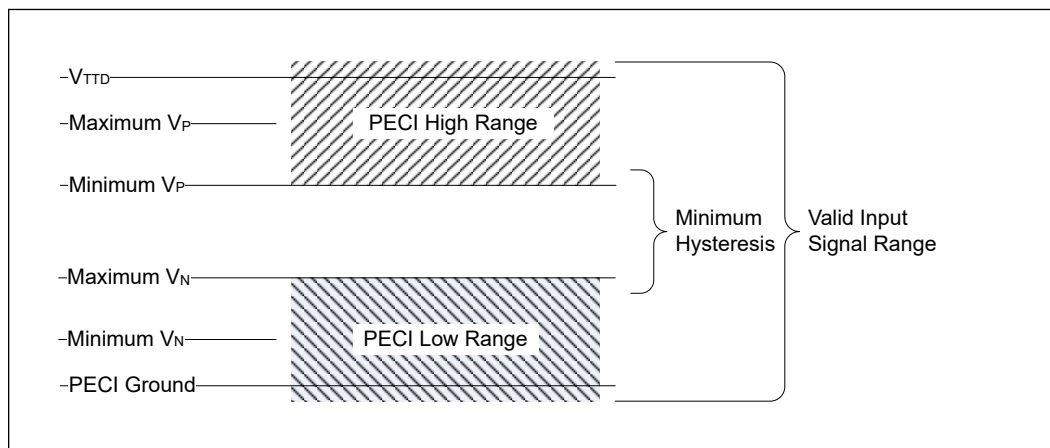
Figure 34. Input Device Hysteresis
