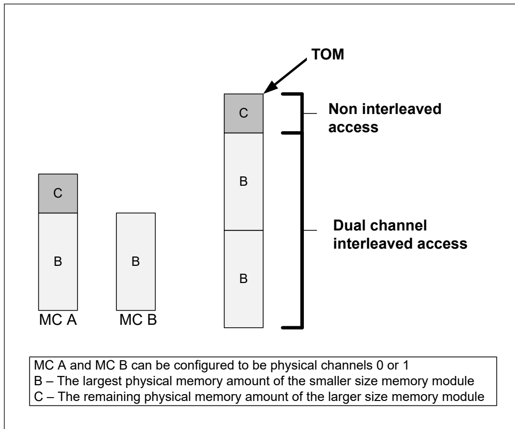
Figure 25. Intel® DDR4/5 Flex Memory Technology Operations
