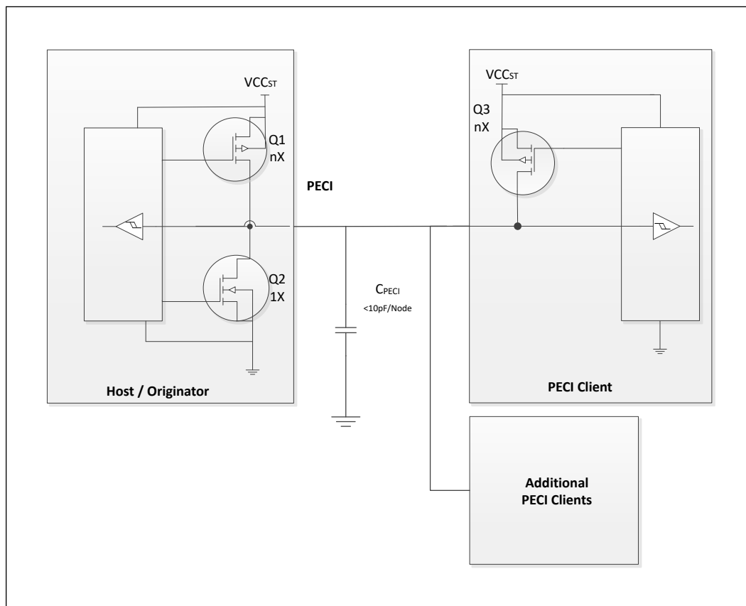
Figure 6. Example for PECI Host-Clients Connection
