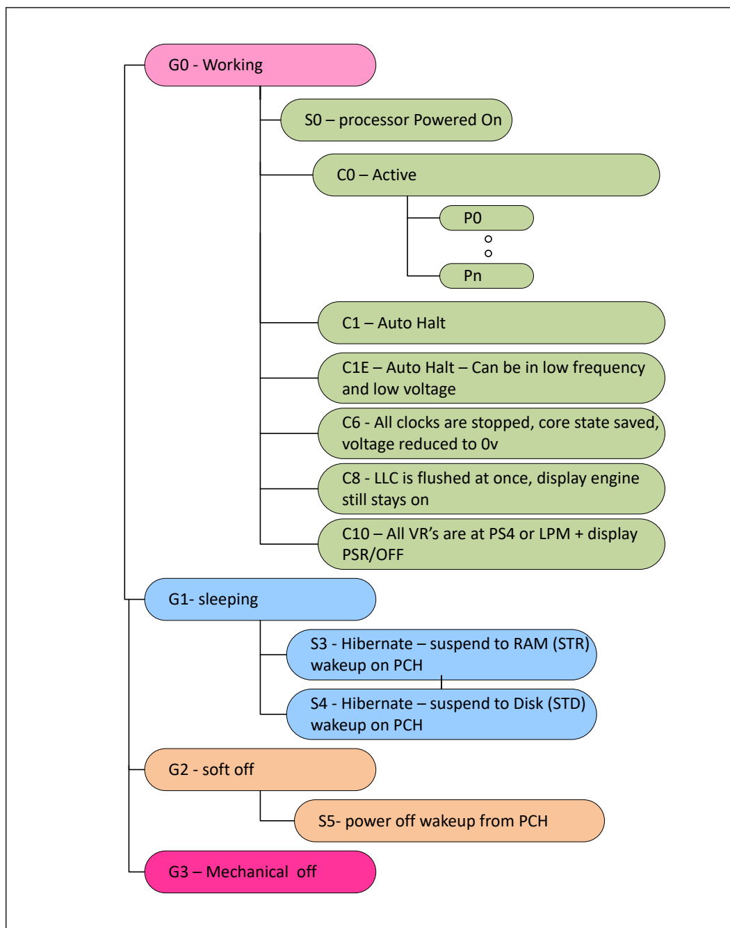
Figure 12. Processor Power States
