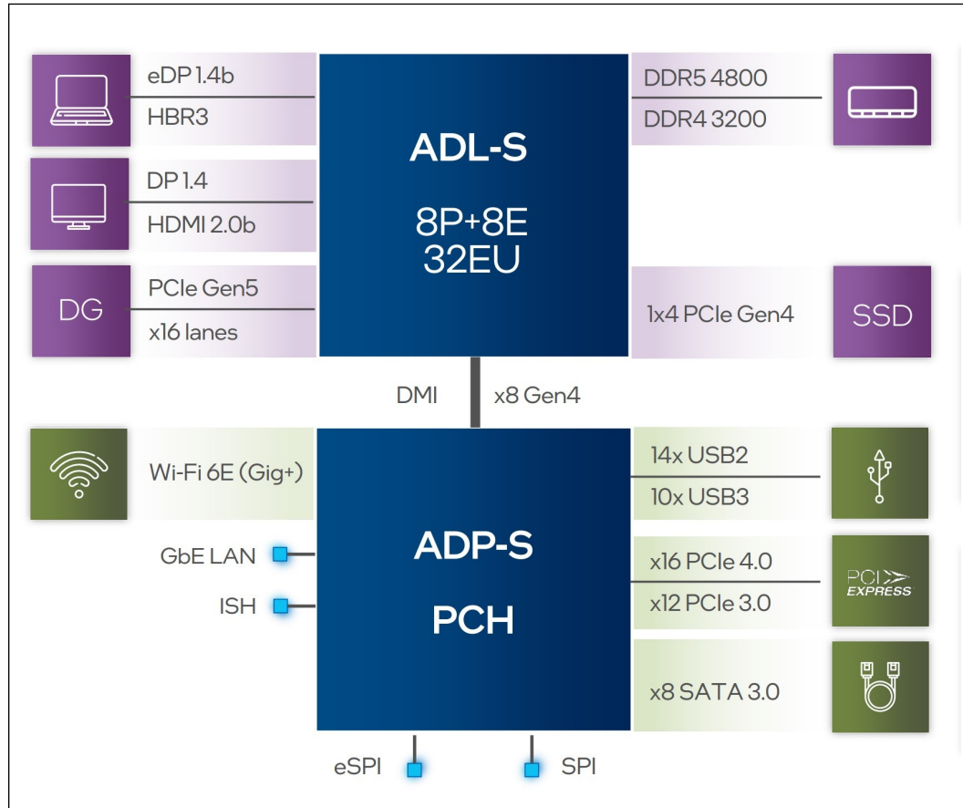
Figure 5. HX Processor Line Platform Diagram
