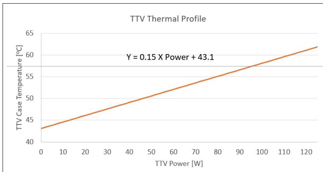
Figure 19. Thermal Profile for PCG 2020A Processor
