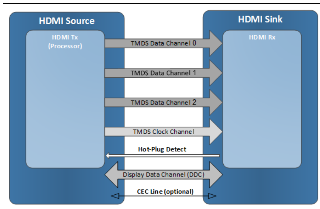
Figure 32. HDMI* Overview
