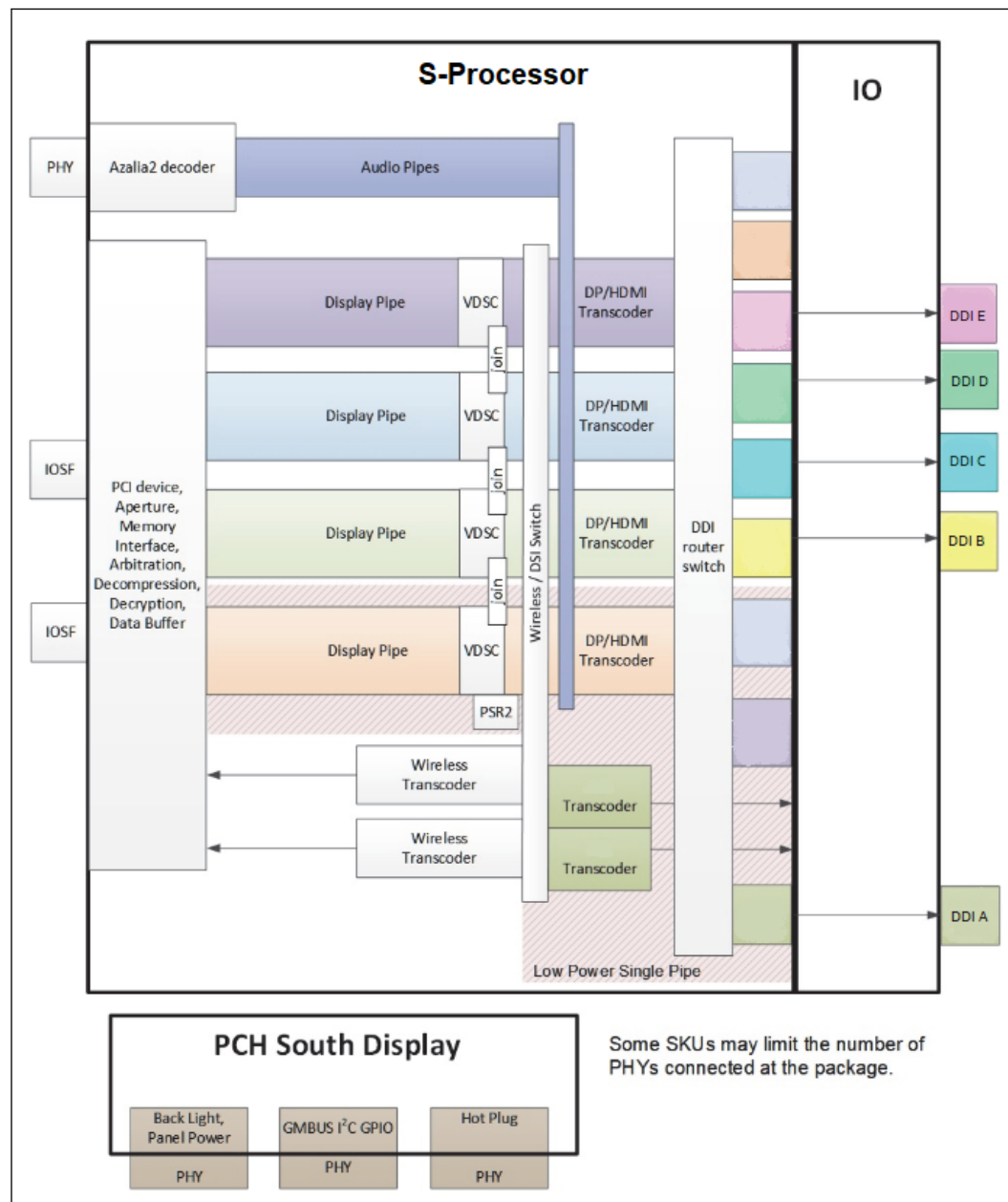
Figure 29. S Processor Display Architecture
