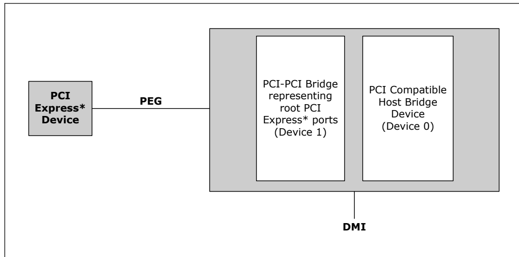
Figure 27. PCI Express® Related Register Structures in the Processor
