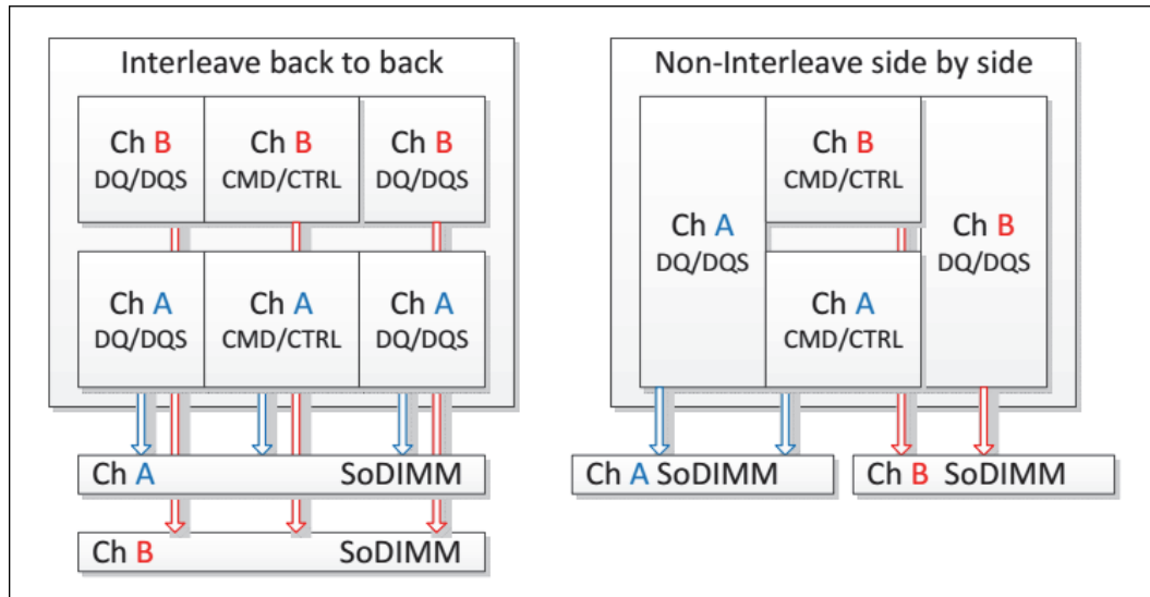
Figure 26. DDR4 Interleave (IL) and Non-Interleave (NIL) Modes Mapping
