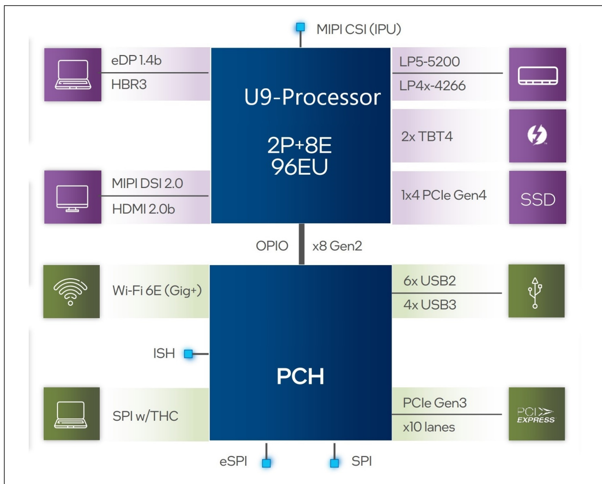
Figure 4. U9 Processor Line Platform Diagram
