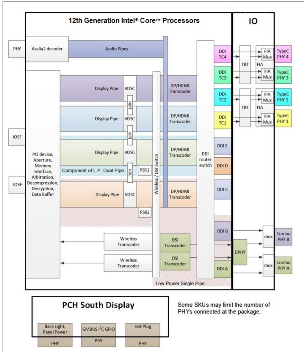
Figure 30. H/P/U Processor Display Architecture
