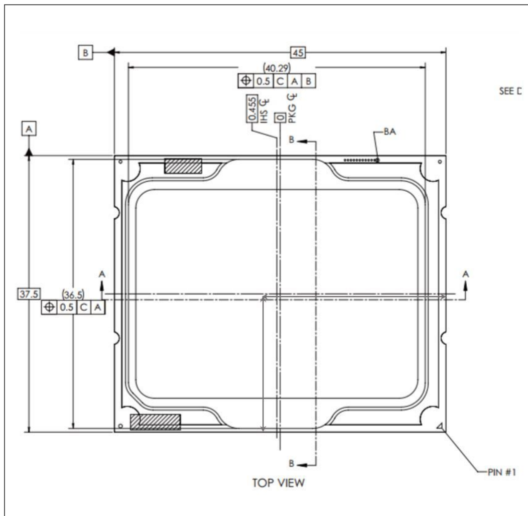
Figure 22. Thermal Test Vehicle (TTV) Case Temperature ( T_{CASE} ) Measurement Location
