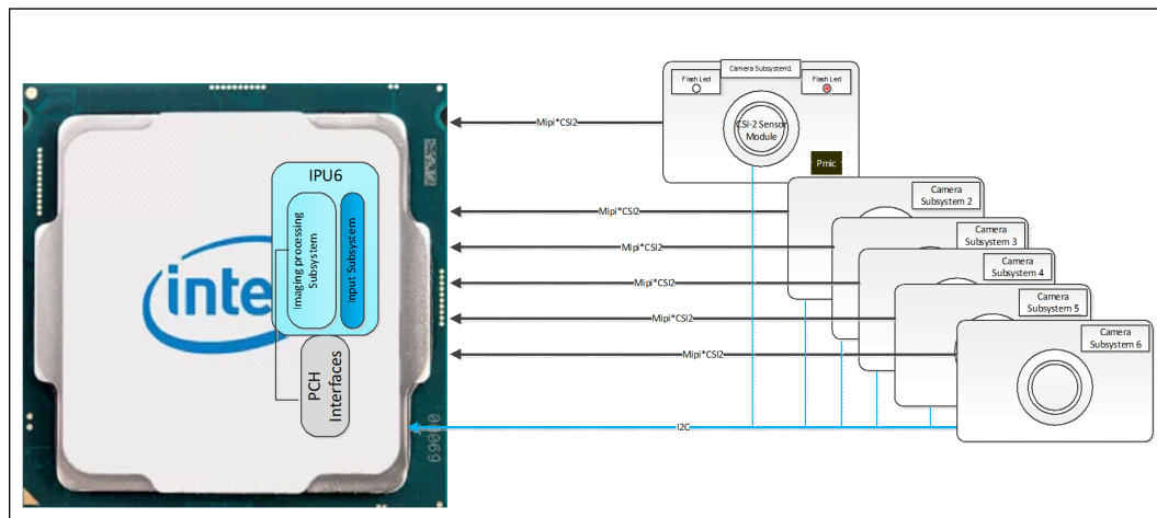
Figure 10. Processor Camera System
