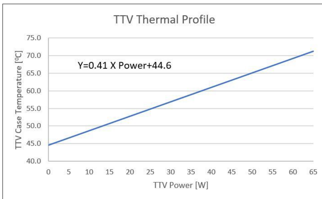
Figure 20. Thermal Profile for PCG 2020C Processor
