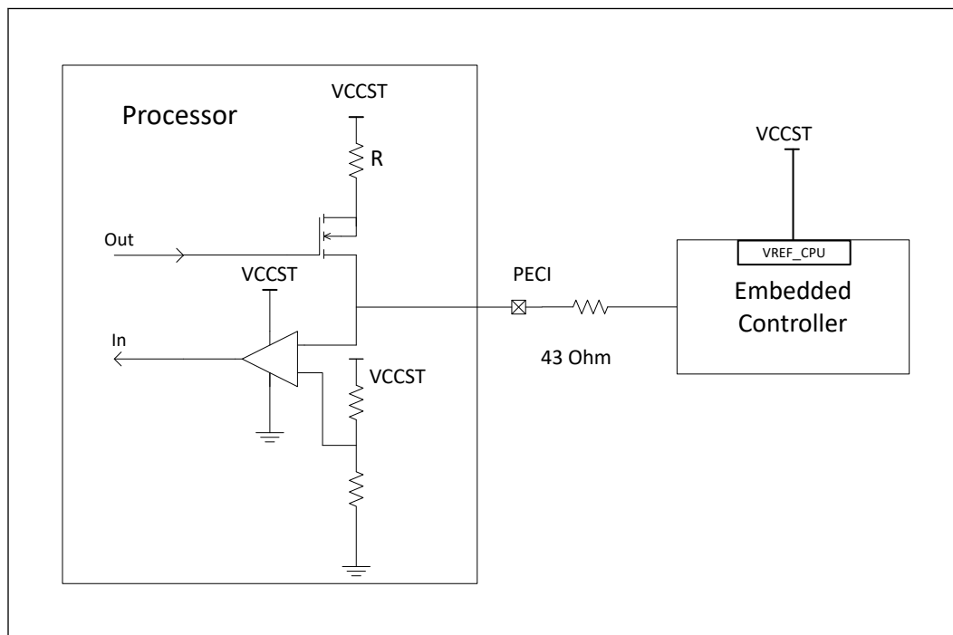
Figure 7. Example for PECI EC Connection
