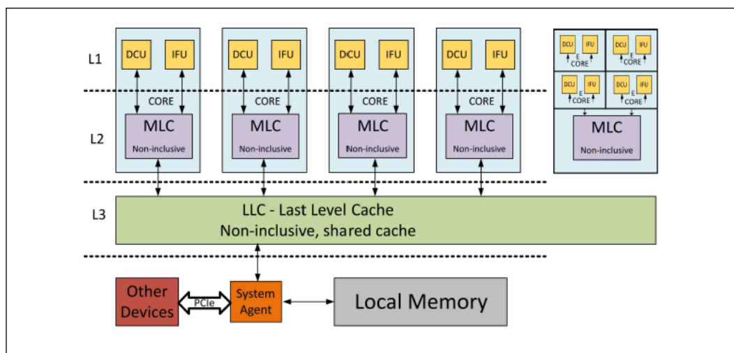
Figure 9. Hybrid Cache
