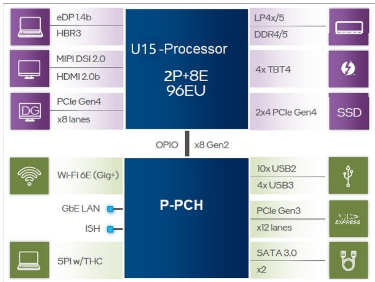
Figure 3. U15 Processor Line Platform Diagram
