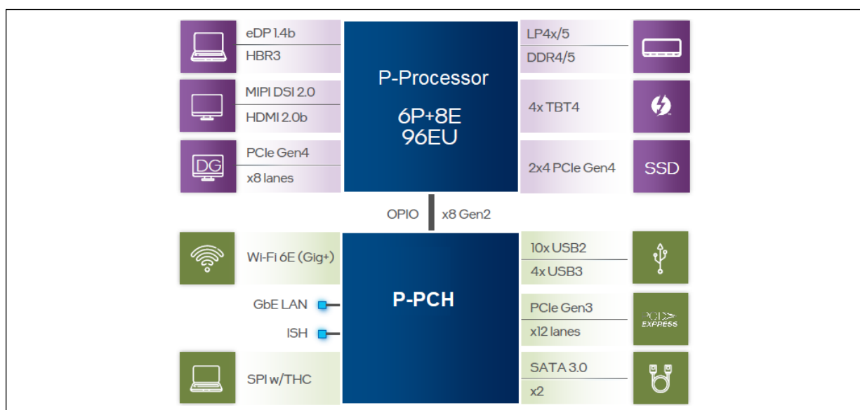
Figure 2. H/P Processor Line Platform Diagram
