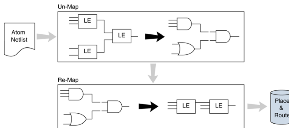
Figure 16-1. WYSIWYG Primitive Resynthesis
