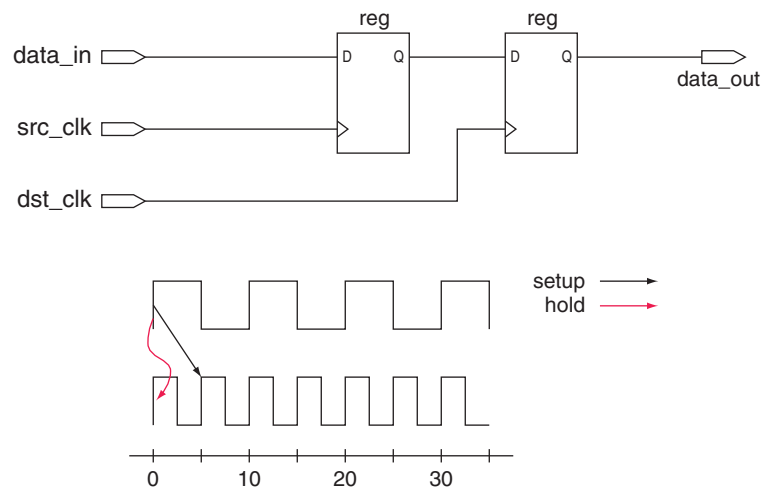
Figure 6-9. Register-to-Register Path and Default Setup and Hold Timing Diagram
