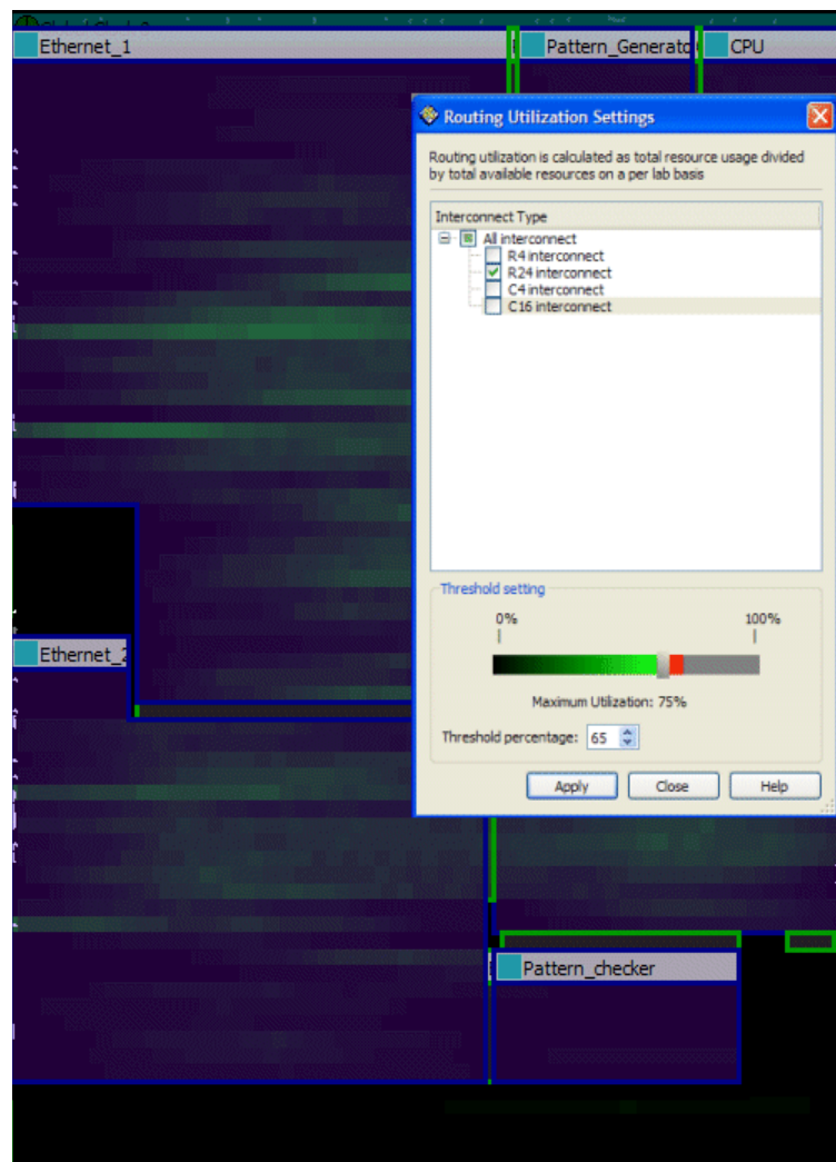
Figure 5-25. Routing Congestion
