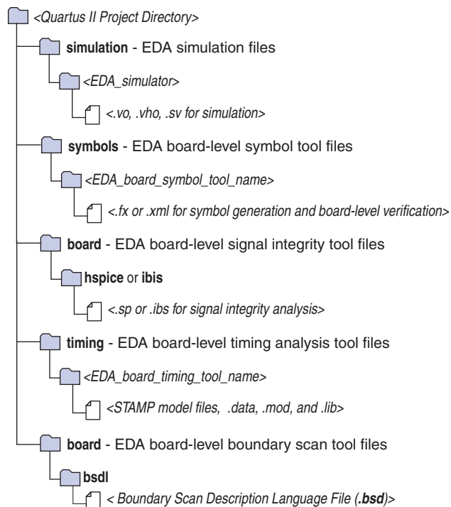
Figure 1–3. Quartus II Generated Files for Other EDA Tools
