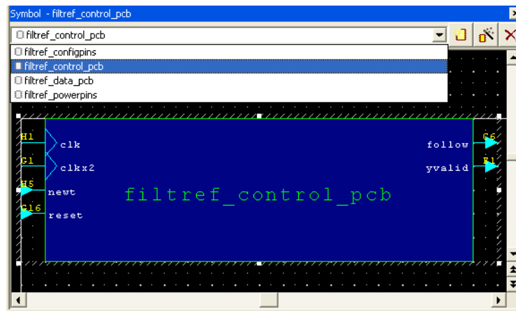
Figure 7-12. The I/O Designer Symbol Editor
