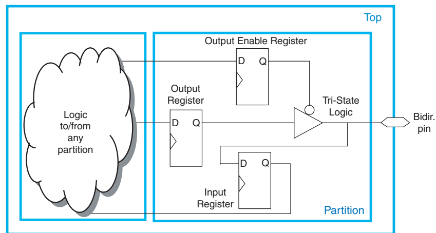
Figure 15-18. Including All Bidirectional I/O Registers in the Same Partition (for Older Devices)
