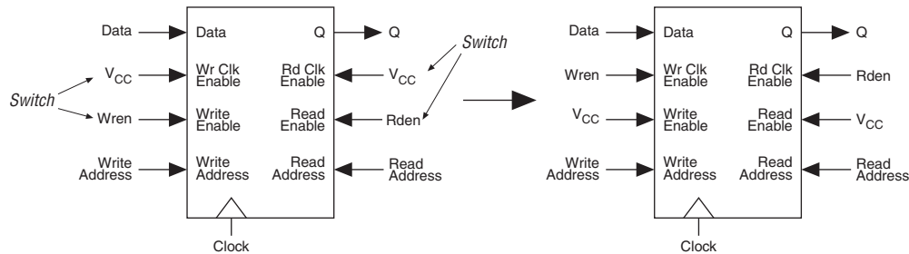
Figure 13–4. Memory Transformation
