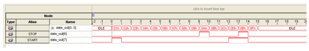
Figure 13-17. Data Acquisition of a Recurring Data Pattern in Continuous Mode (to illustrate Start/Stop mode)
