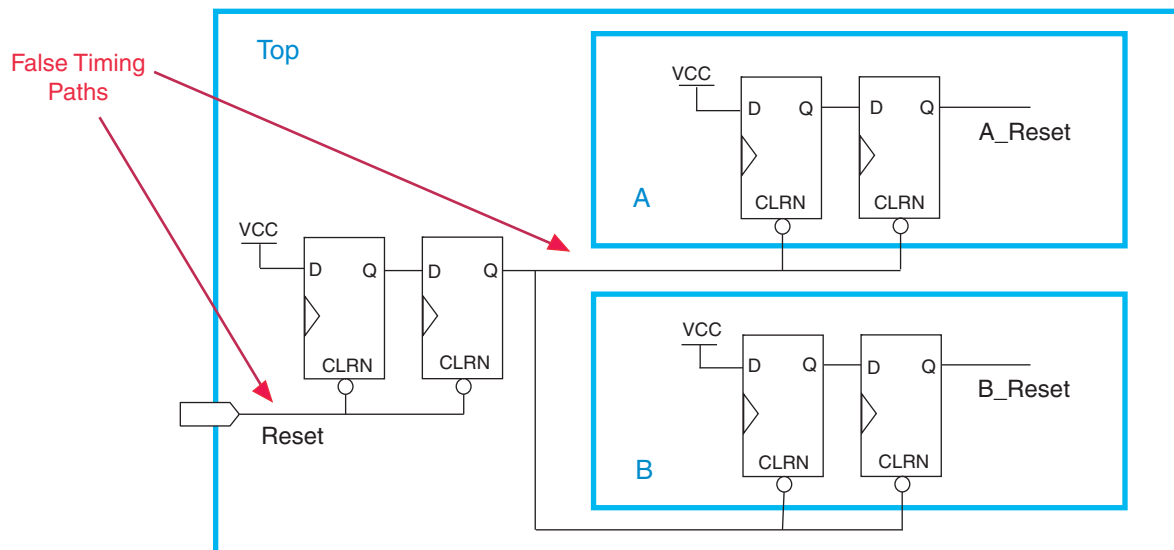
Figure 15-19. Cascaded Reset Structure
