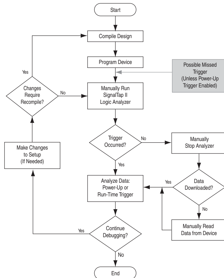
Figure 13-35. Power-Up and Runtime Trigger Events Flowchart
