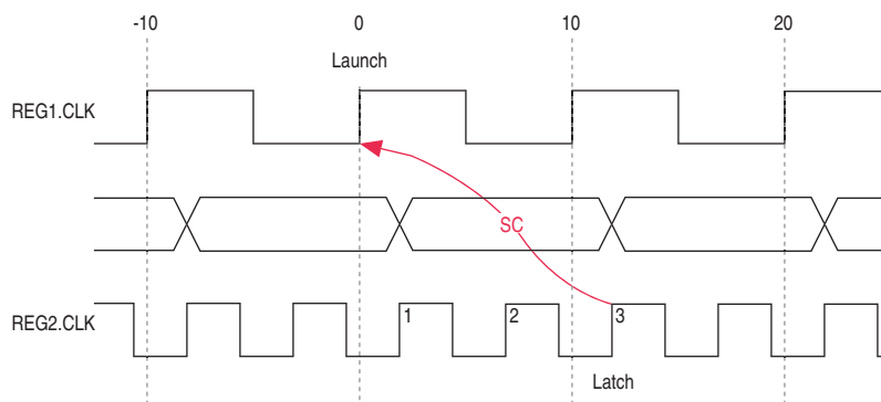
Figure 7-43. Preferred Setup Analysis
