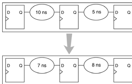
Figure 16-2. Register Retiming Diagram
