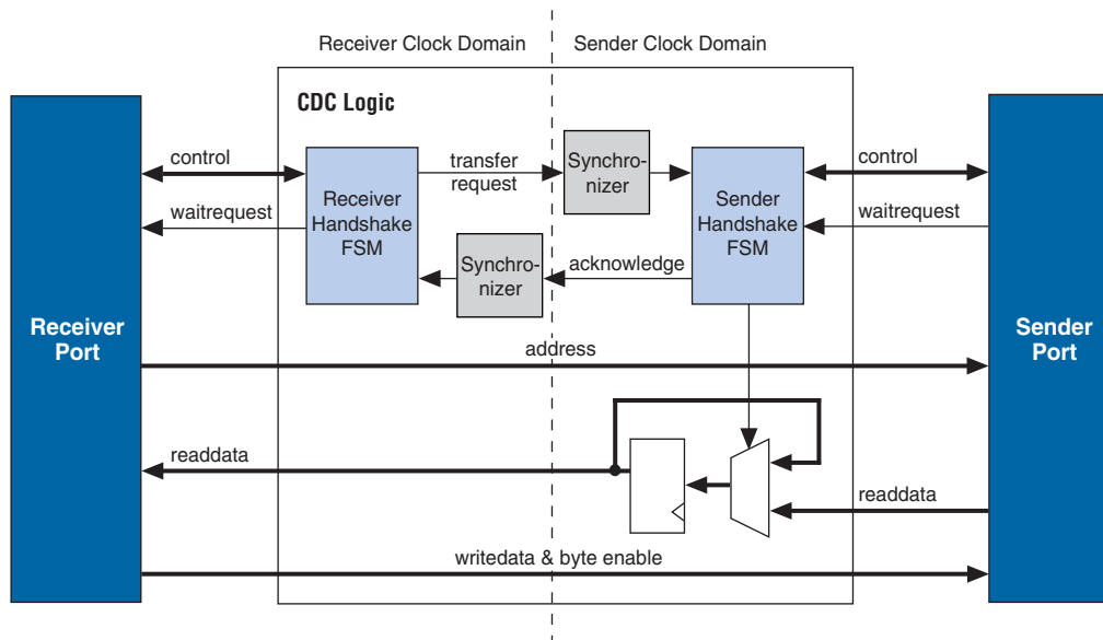
Figure 9-23. Block Diagram of Clock Crossing Adapter
