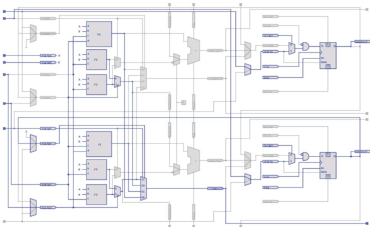
Figure 17-5. ALM Schematic (1)
