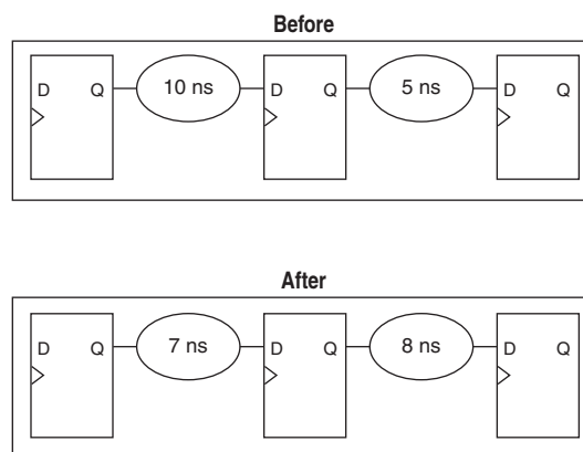
Figure 13-7. Gate-Level Register Retiming
