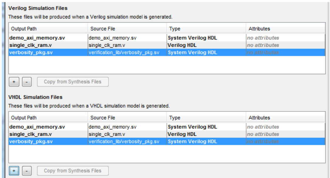
Figure 7-3: Specifying the Simulation Output Files
