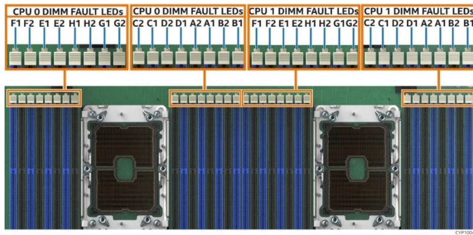
Figure 103. Memory Fault LED Location
