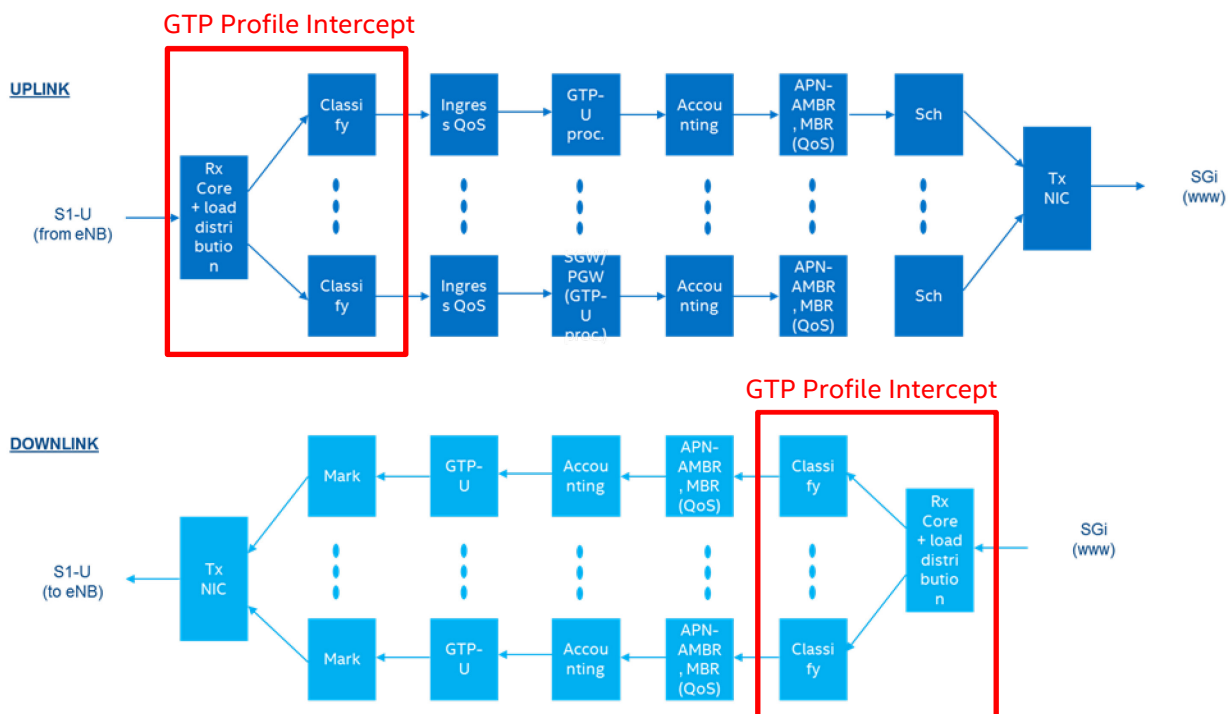
Figure 6: Typical vEPC server node packet pipeline
