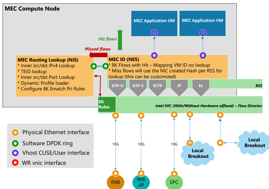
Figure 12: DDP offload on NEV SDK for MEC S1 interface
