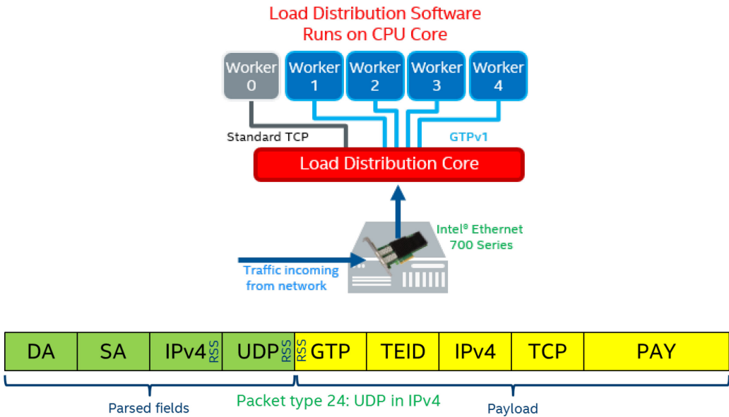
Figure 2: Packet header identification before application of GTPv1 profile
