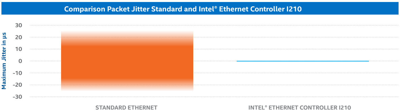
Figure 3. Comparison of packet jitter between SoftMaster* implemented with Standard PC Ethernet interface and PC with Intel® I210 interface.
